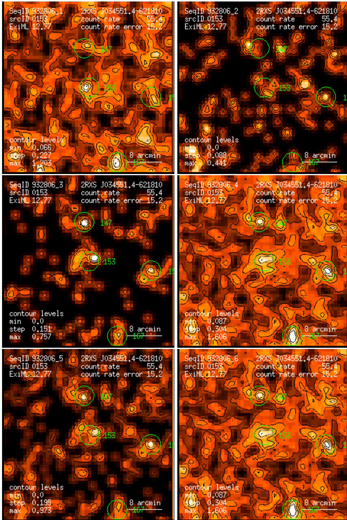
Figure 153: RASS 932806: detection 0153: band rate images, Gaussian filter: (1) PSPC channels 11 – 41, (2) 52 – 90, (3) 91 – 201, (4) 11 – 235, (5) 52 – 201, (6) 11 – 201. Broad band rates in counts/ks. Band rate contour levels in counts/ks/arcmin 2 .
