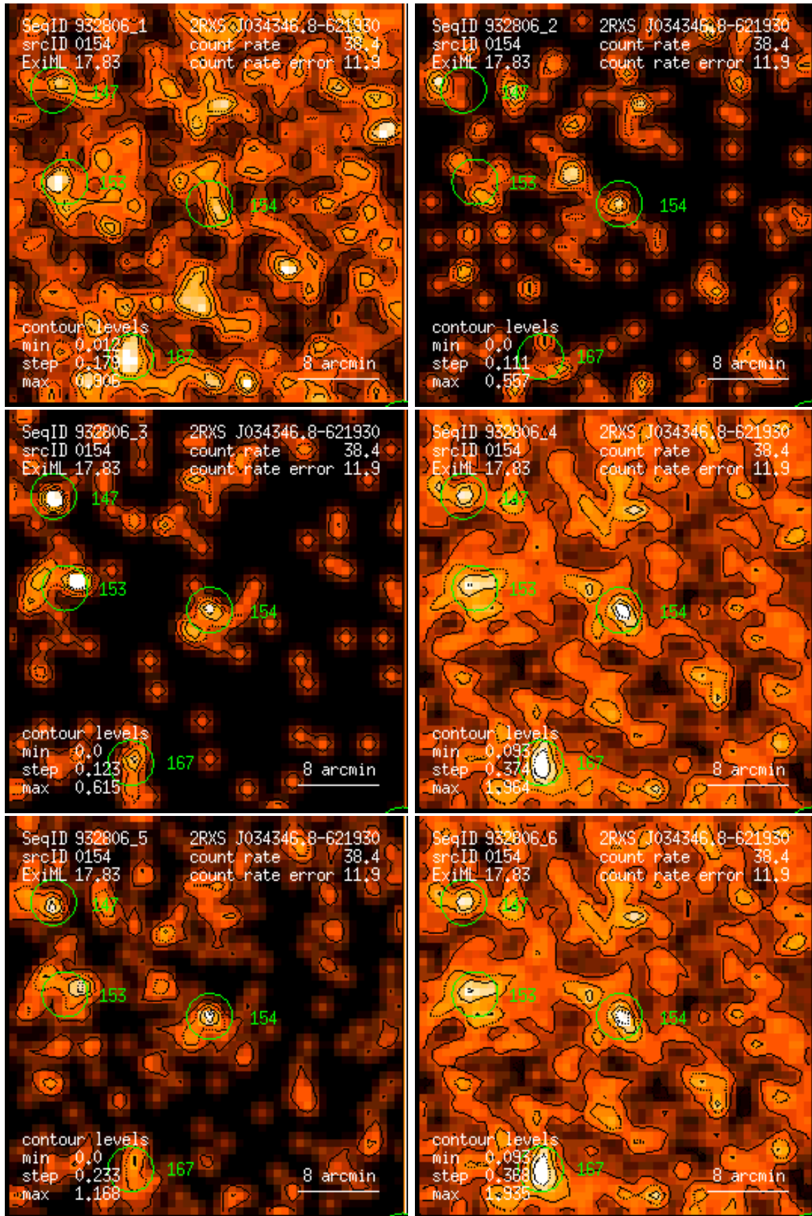
Figure 154: RASS 932806: detection 0154: band rate images, Gaussian filter: (1) PSPC channels 11 – 41, (2) 52 – 90, (3) 91 – 201, (4) 11 – 235, (5) 52 – 201, (6) 11 – 201. Broad band rates in counts/ks. Band rate contour levels in counts/ks/arcmin 2 .
