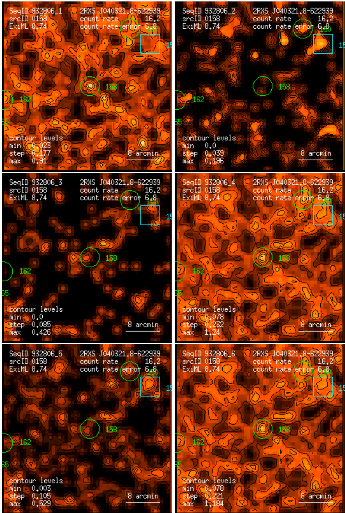
Figure 158: RASS 932806: detection 0158: band rate images, Gaussian filter: (1) PSPC channels 11 – 41, (2) 52 – 90, (3) 91 – 201, (4) 11 – 235, (5) 52 – 201, (6) 11 – 201. Broad band rates in counts/ks. Band rate contour levels in counts/ks/arcmin 2 .
