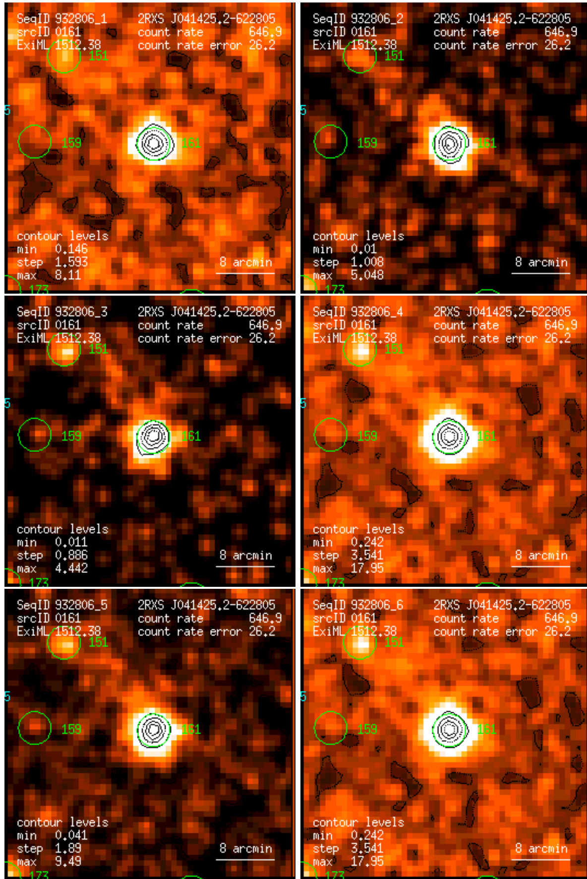
Figure 161: RASS 932806: detection 0161: band rate images, Gaussian filter: (1) PSPC channels 11 – 41, (2) 52 – 90, (3) 91 – 201, (4) 11 – 235, (5) 52 – 201, (6) 11 – 201. Broad band rates in counts/ks. Band rate contour levels in counts/ks/arcmin 2 .
