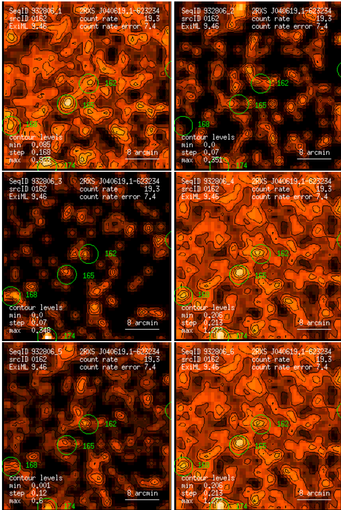
Figure 162: RASS 932806: detection 0162: band rate images, Gaussian filter: (1) PSPC channels 11 – 41, (2) 52 – 90, (3) 91 – 201, (4) 11 – 235, (5) 52 – 201, (6) 11 – 201. Broad band rates in counts/ks. Band rate contour levels in counts/ks/arcmin 2 .
