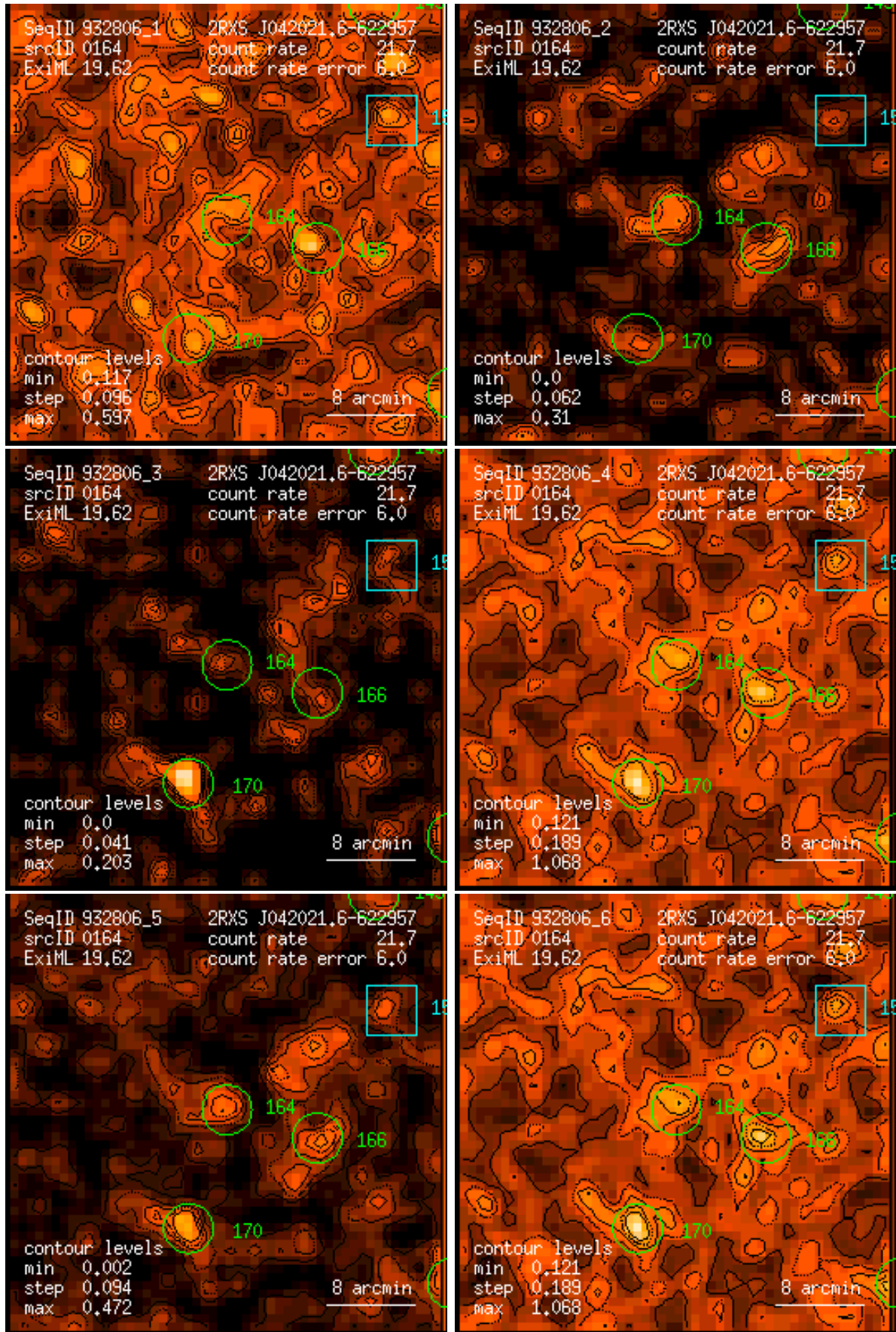
Figure 164: RASS 932806: detection 0164: band rate images, Gaussian filter: (1) PSPC channels 11 – 41, (2) 52 – 90, (3) 91 – 201, (4) 11 – 235, (5) 52 – 201, (6) 11 – 201. Broad band rates in counts/ks. Band rate contour levels in counts/ks/arcmin 2 .
