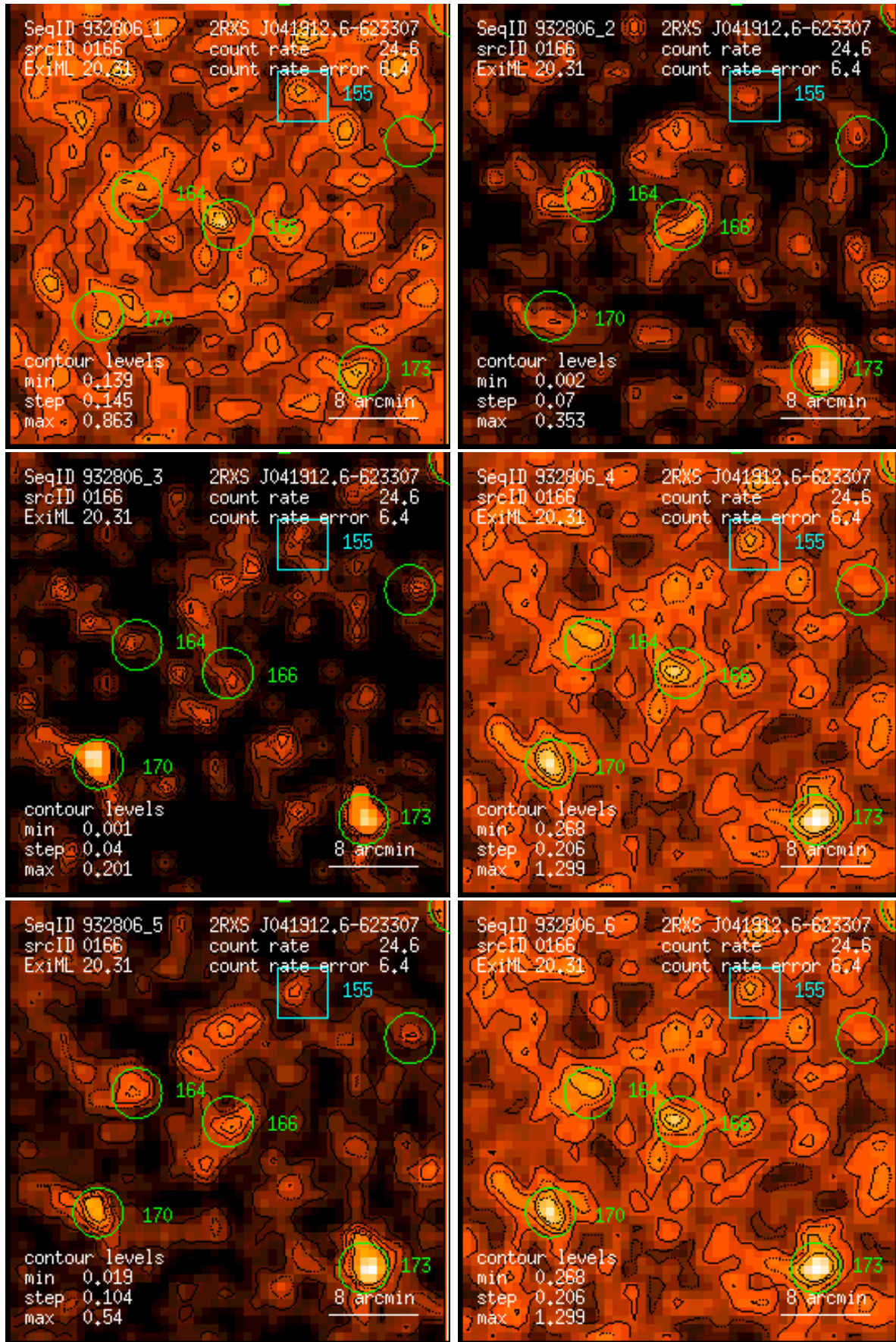
Figure 166: RASS 932806: detection 0166: band rate images, Gaussian filter: (1) PSPC channels 11 – 41, (2) 52 – 90, (3) 91 – 201, (4) 11 – 235, (5) 52 – 201, (6) 11 – 201. Broad band rates in counts/ks. Band rate contour levels in counts/ks/arcmin 2 .
