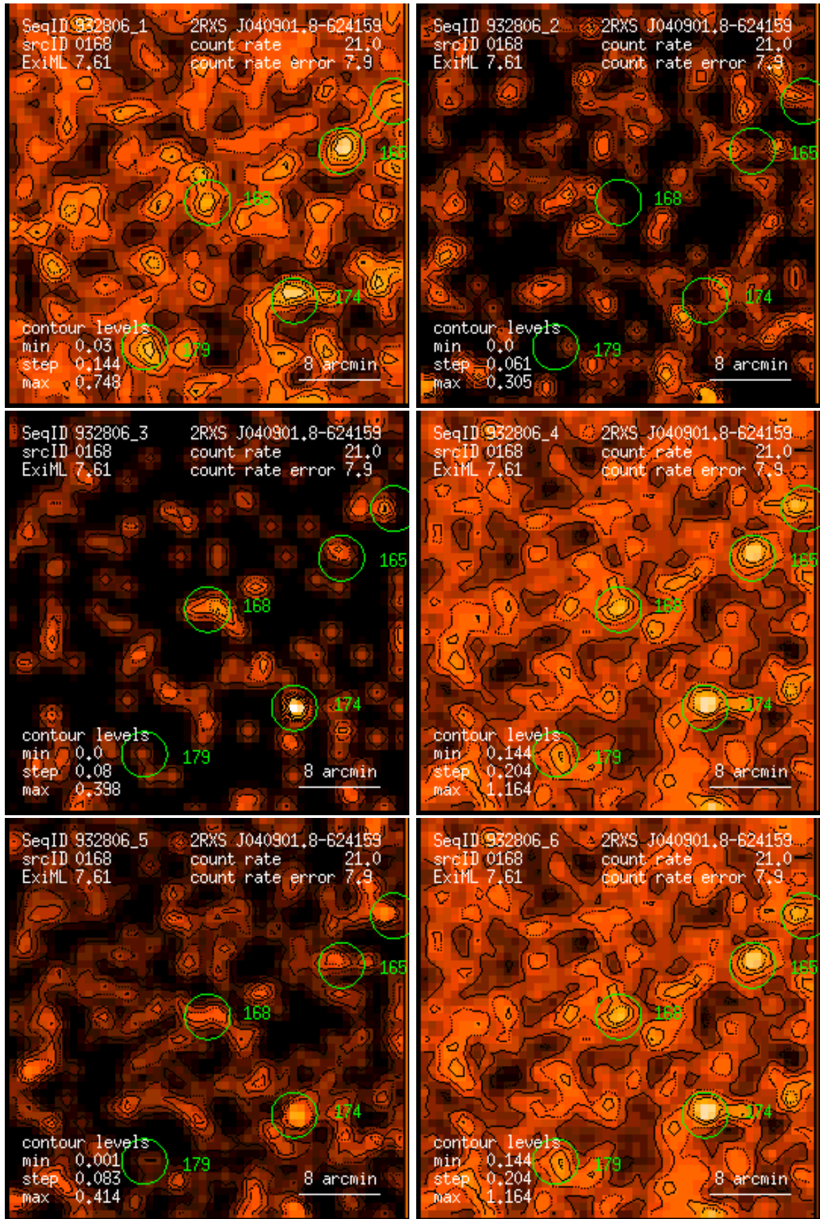
Figure 168: RASS 932806: detection 0168: band rate images, Gaussian filter: (1) PSPC channels 11 – 41, (2) 52 – 90, (3) 91 – 201, (4) 11 – 235, (5) 52 – 201, (6) 11 – 201. Broad band rates in counts/ks. Band rate contour levels in counts/ks/arcmin 2 .
