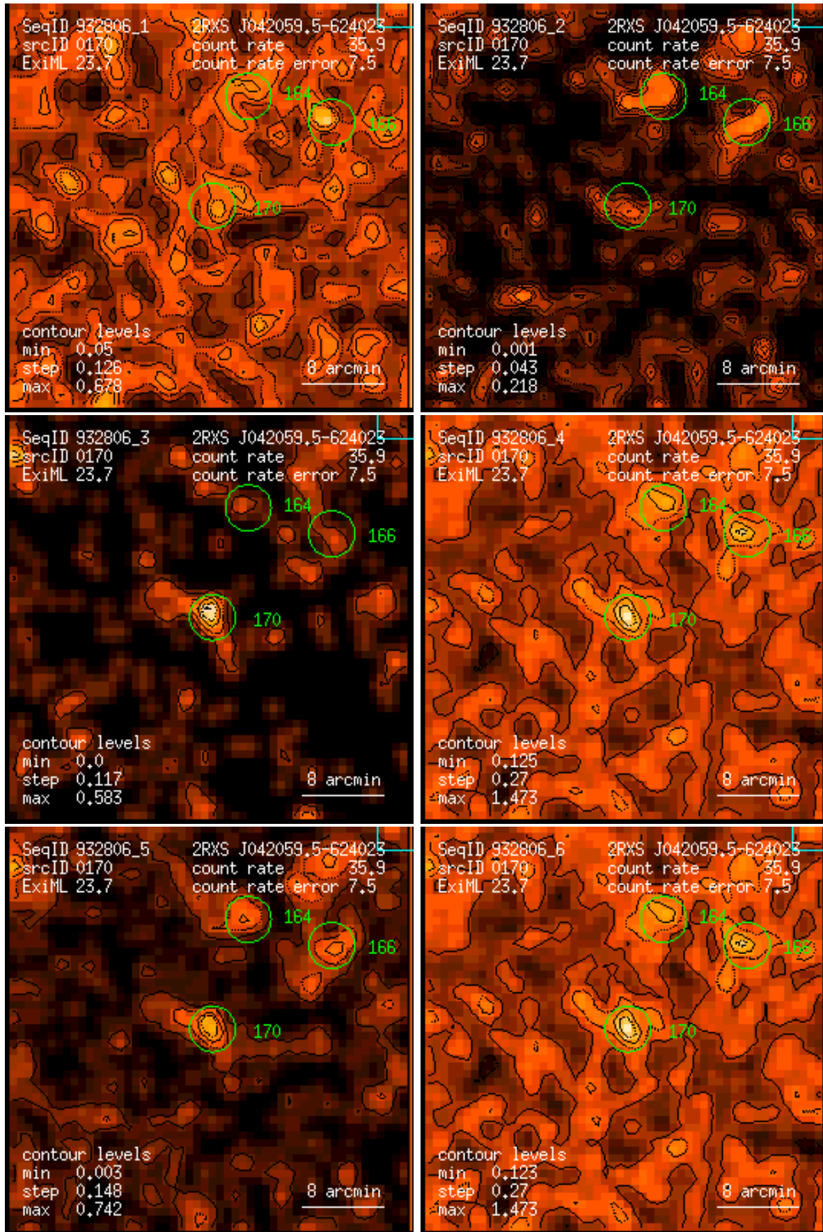
Figure 170: RASS 932806: detection 0170: band rate images, Gaussian filter: (1) PSPC channels 11 – 41, (2) 52 – 90, (3) 91 – 201, (4) 11 – 235, (5) 52 – 201, (6) 11 – 201. Broad band rates in counts/ks. Band rate contour levels in counts/ks/arcmin 2 .
