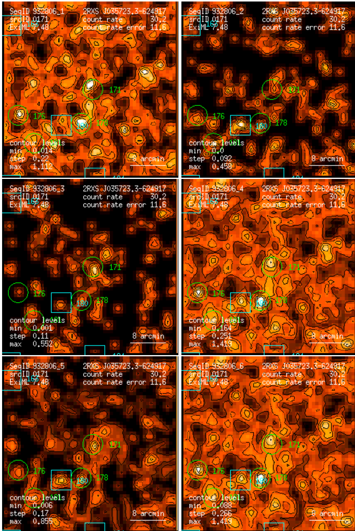
Figure 171: RASS 932806: detection 0171: band rate images, Gaussian filter: (1) PSPC channels 11 – 41, (2) 52 – 90, (3) 91 – 201, (4) 11 – 235, (5) 52 – 201, (6) 11 – 201. Broad band rates in counts/ks. Band rate contour levels in counts/ks/arcmin 2 .
