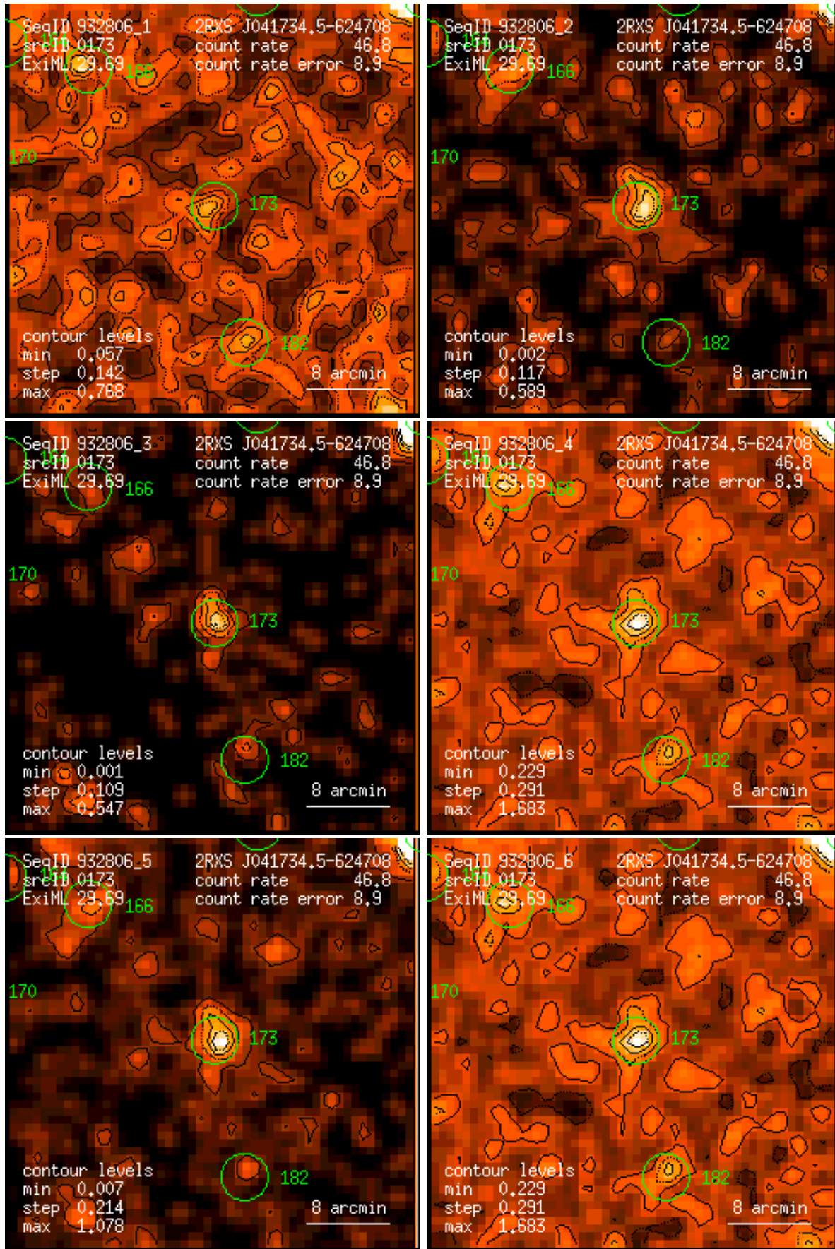
Figure 173: RASS 932806: detection 0173: band rate images, Gaussian filter: (1) PSPC channels 11 – 41, (2) 52 – 90, (3) 91 – 201, (4) 11 – 235, (5) 52 – 201, (6) 11 – 201. Broad band rates in counts/ks. Band rate contour levels in counts/ks/arcmin 2 .
