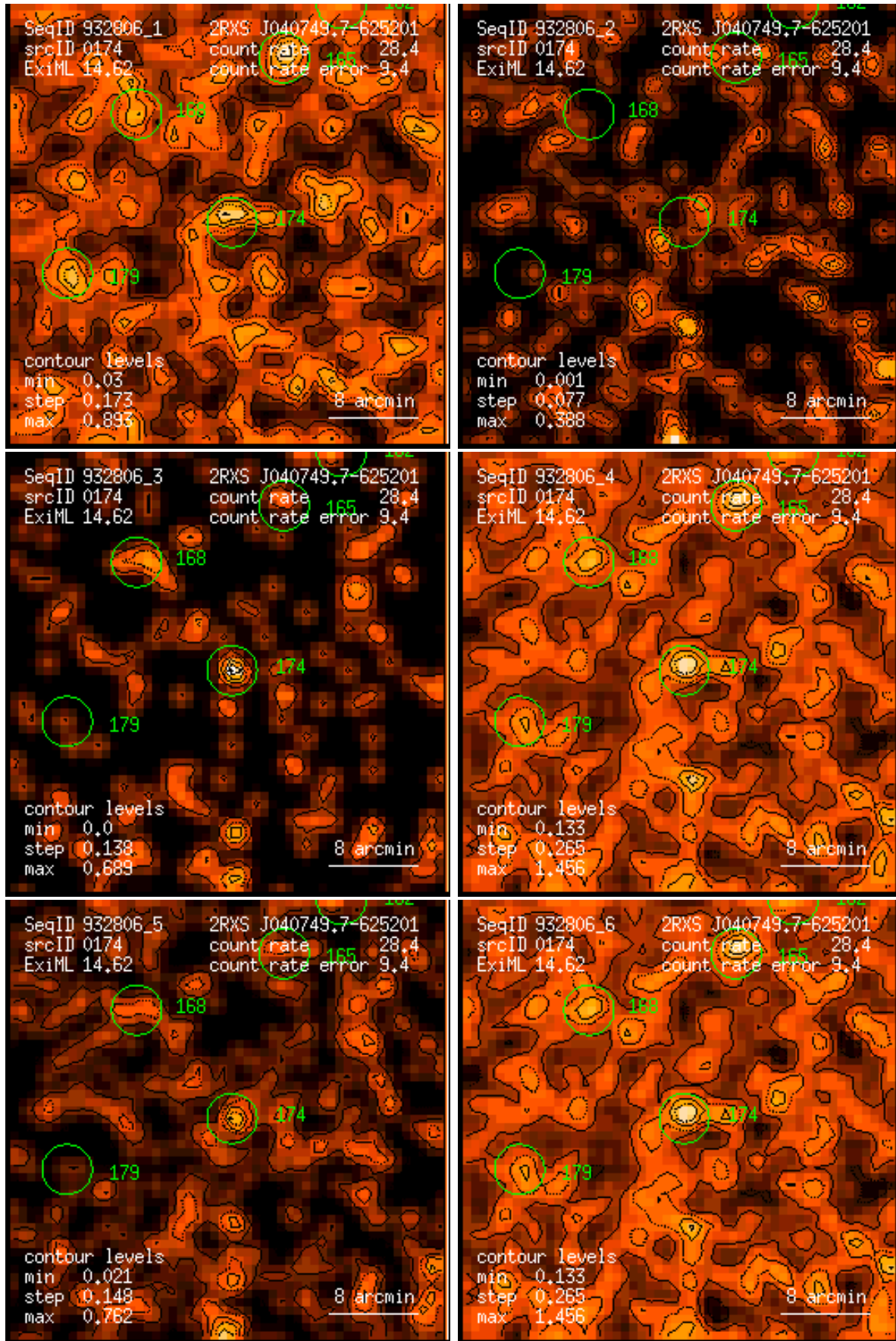
Figure 174: RASS 932806: detection 0174: band rate images, Gaussian filter: (1) PSPC channels 11 – 41, (2) 52 – 90, (3) 91 – 201, (4) 11 – 235, (5) 52 – 201, (6) 11 – 201. Broad band rates in counts/ks. Band rate contour levels in counts/ks/arcmin 2 .
