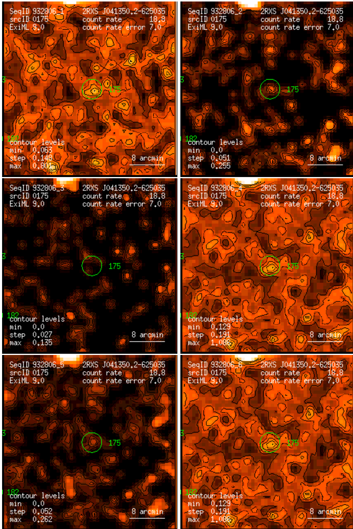
Figure 175: RASS 932806: detection 0175: band rate images, Gaussian filter: (1) PSPC channels 11 – 41, (2) 52 – 90, (3) 91 – 201, (4) 11 – 235, (5) 52 – 201, (6) 11 – 201. Broad band rates in counts/ks. Band rate contour levels in counts/ks/arcmin 2 .
