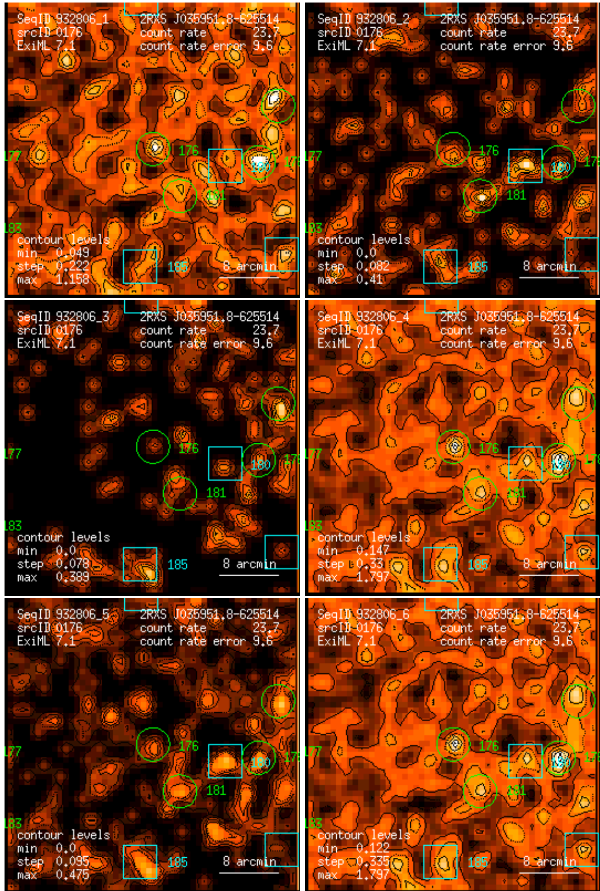
Figure 176: RASS 932806: detection 0176: band rate images, Gaussian filter: (1) PSPC channels 11 – 41, (2) 52 – 90, (3) 91 – 201, (4) 11 – 235, (5) 52 – 201, (6) 11 – 201. Broad band rates in counts/ks. Band rate contour levels in counts/ks/arcmin 2 .
