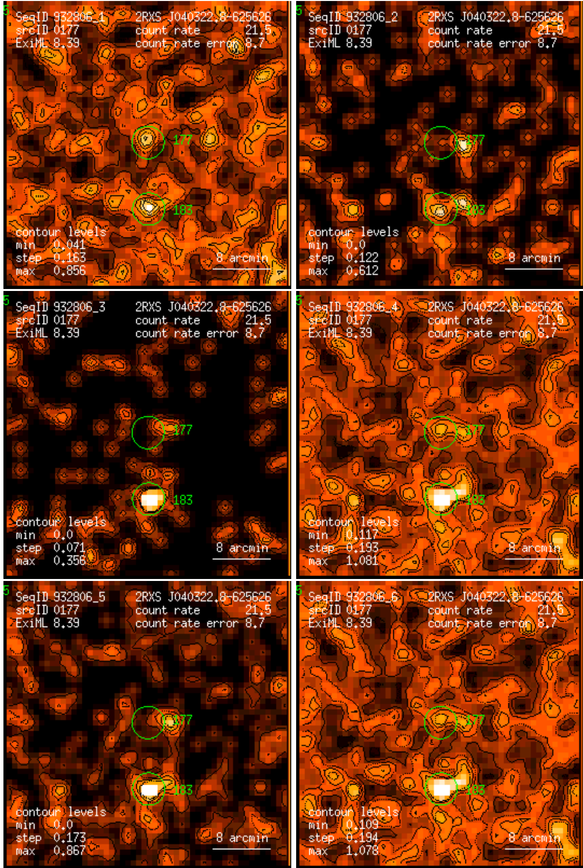
Figure 177: RASS 932806: detection 0177: band rate images, Gaussian filter: (1) PSPC channels 11 – 41, (2) 52 – 90, (3) 91 – 201, (4) 11 – 235, (5) 52 – 201, (6) 11 – 201. Broad band rates in counts/ks. Band rate contour levels in counts/ks/arcmin 2 .
