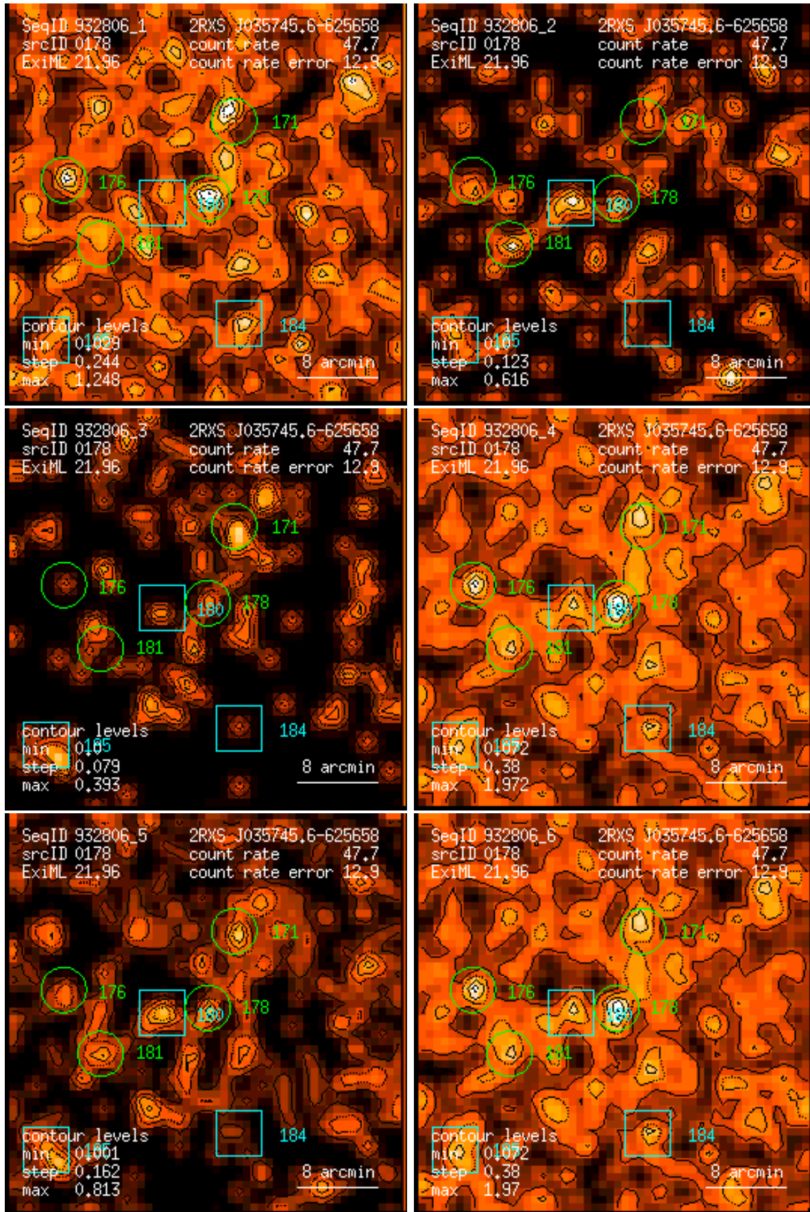
Figure 178: RASS 932806: detection 0178: band rate images, Gaussian filter: (1) PSPC channels 11 – 41, (2) 52 – 90, (3) 91 – 201, (4) 11 – 235, (5) 52 – 201, (6) 11 – 201. Broad band rates in counts/ks. Band rate contour levels in counts/ks/arcmin 2 .
