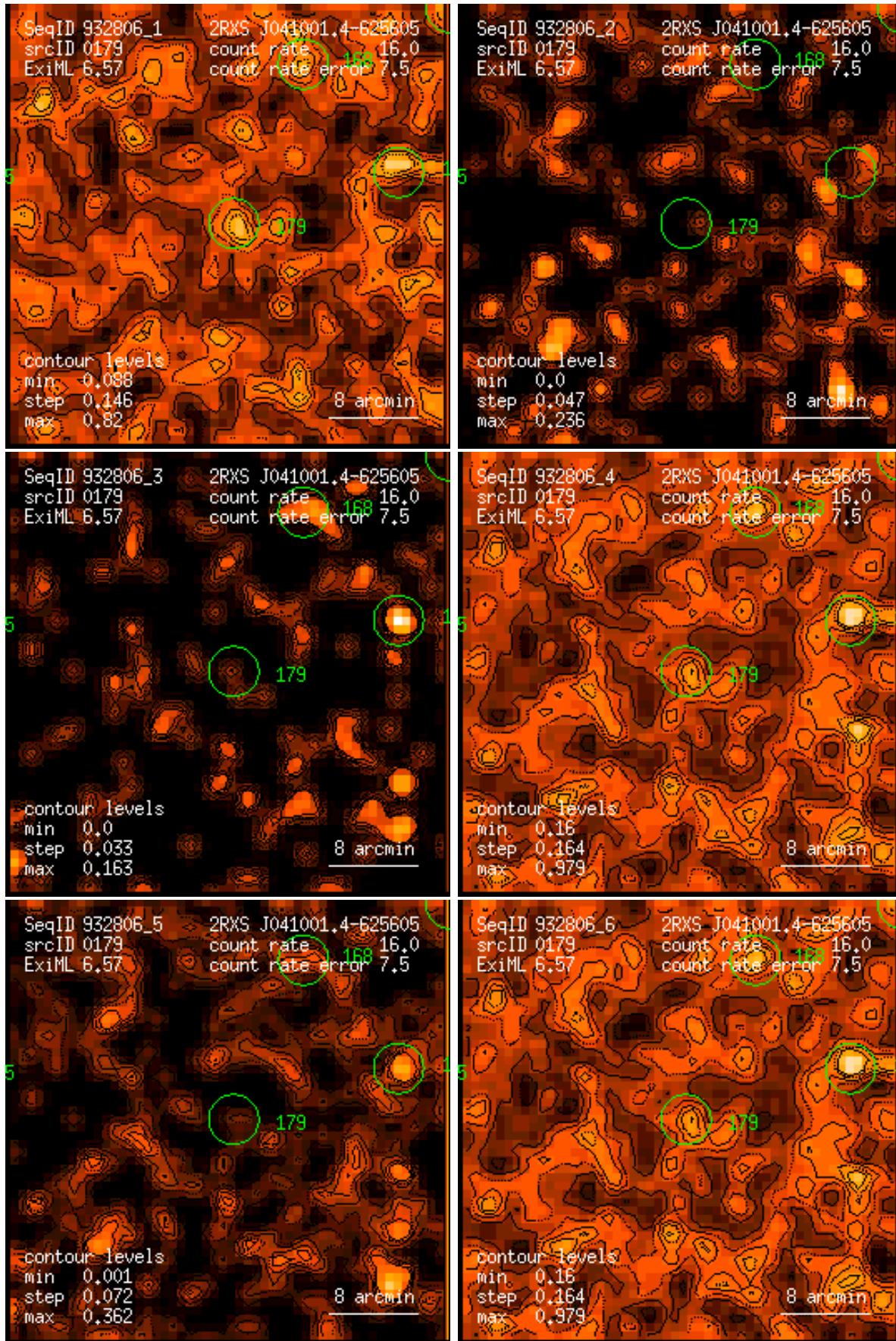
Figure 179: RASS 932806: detection 0179: band rate images, Gaussian filter: (1) PSPC channels 11 – 41, (2) 52 – 90, (3) 91 – 201, (4) 11 – 235, (5) 52 – 201, (6) 11 – 201. Broad band rates in counts/ks. Band rate contour levels in counts/ks/arcmin 2 .
