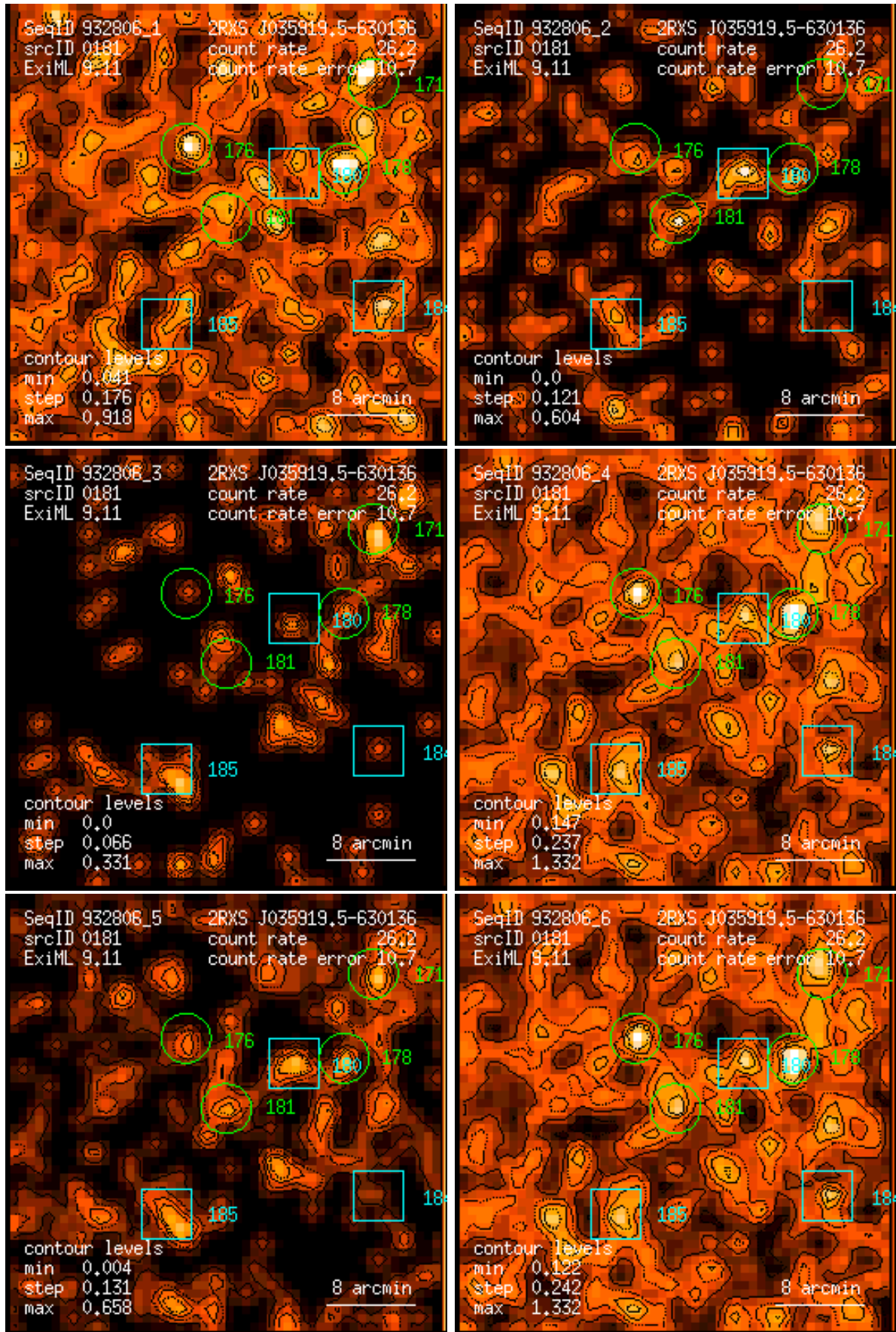
Figure 181: RASS 932806: detection 0181: band rate images, Gaussian filter: (1) PSPC channels 11 – 41, (2) 52 – 90, (3) 91 – 201, (4) 11 – 235, (5) 52 – 201, (6) 11 – 201. Broad band rates in counts/ks. Band rate contour levels in counts/ks/arcmin 2 .
