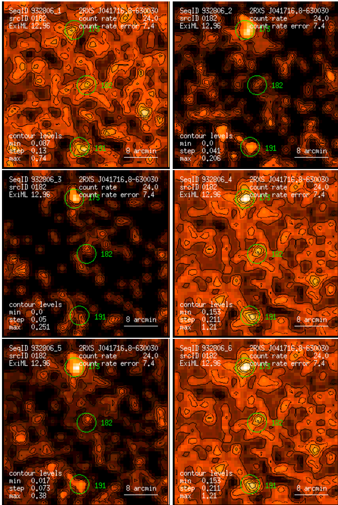
Figure 182: RASS 932806: detection 0182: band rate images, Gaussian filter: (1) PSPC channels 11 – 41, (2) 52 – 90, (3) 91 – 201, (4) 11 – 235, (5) 52 – 201, (6) 11 – 201. Broad band rates in counts/ks. Band rate contour levels in counts/ks/arcmin 2 .
