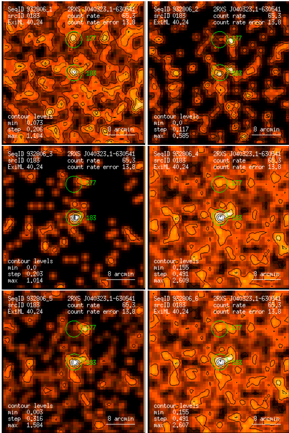
Figure 183: RASS 932806: detection 0183: band rate images, Gaussian filter: (1) PSPC channels 11 – 41, (2) 52 – 90, (3) 91 – 201, (4) 11 – 235, (5) 52 – 201, (6) 11 – 201. Broad band rates in counts/ks. Band rate contour levels in counts/ks/arcmin 2 .
