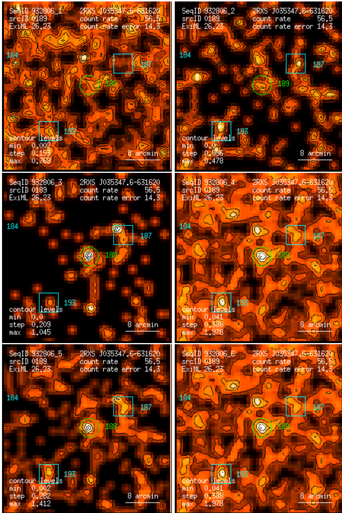
Figure 189: RASS 932806: detection 0189: band rate images, Gaussian filter: (1) PSPC channels 11 – 41, (2) 52 – 90, (3) 91 – 201, (4) 11 – 235, (5) 52 – 201, (6) 11 – 201. Broad band rates in counts/ks. Band rate contour levels in counts/ks/arcmin 2 .
