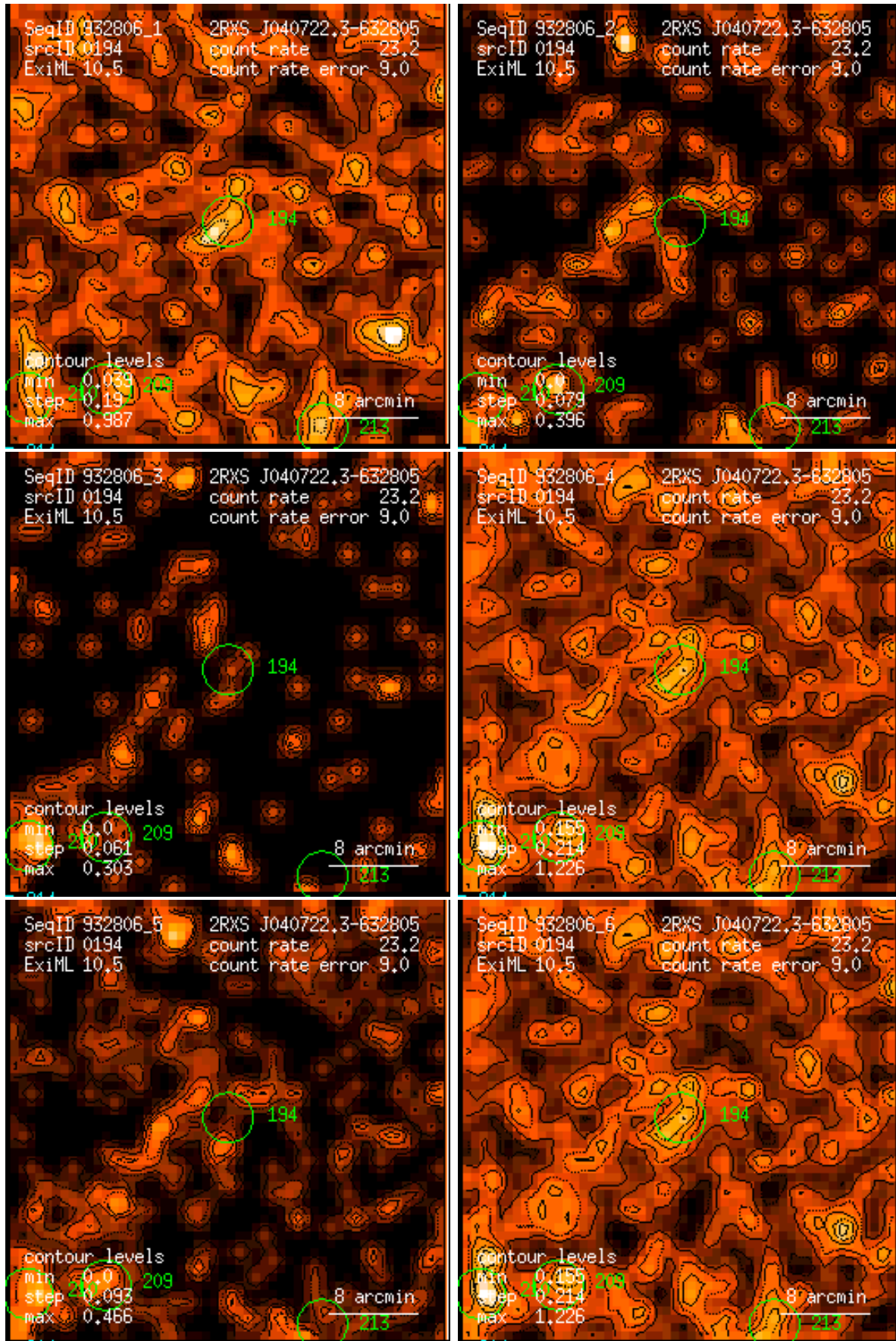
Figure 194: RASS 932806: detection 0194: band rate images, Gaussian filter: (1) PSPC channels 11 – 41, (2) 52 – 90, (3) 91 – 201, (4) 11 – 235, (5) 52 – 201, (6) 11 – 201. Broad band rates in counts/ks. Band rate contour levels in counts/ks/arcmin 2 .
