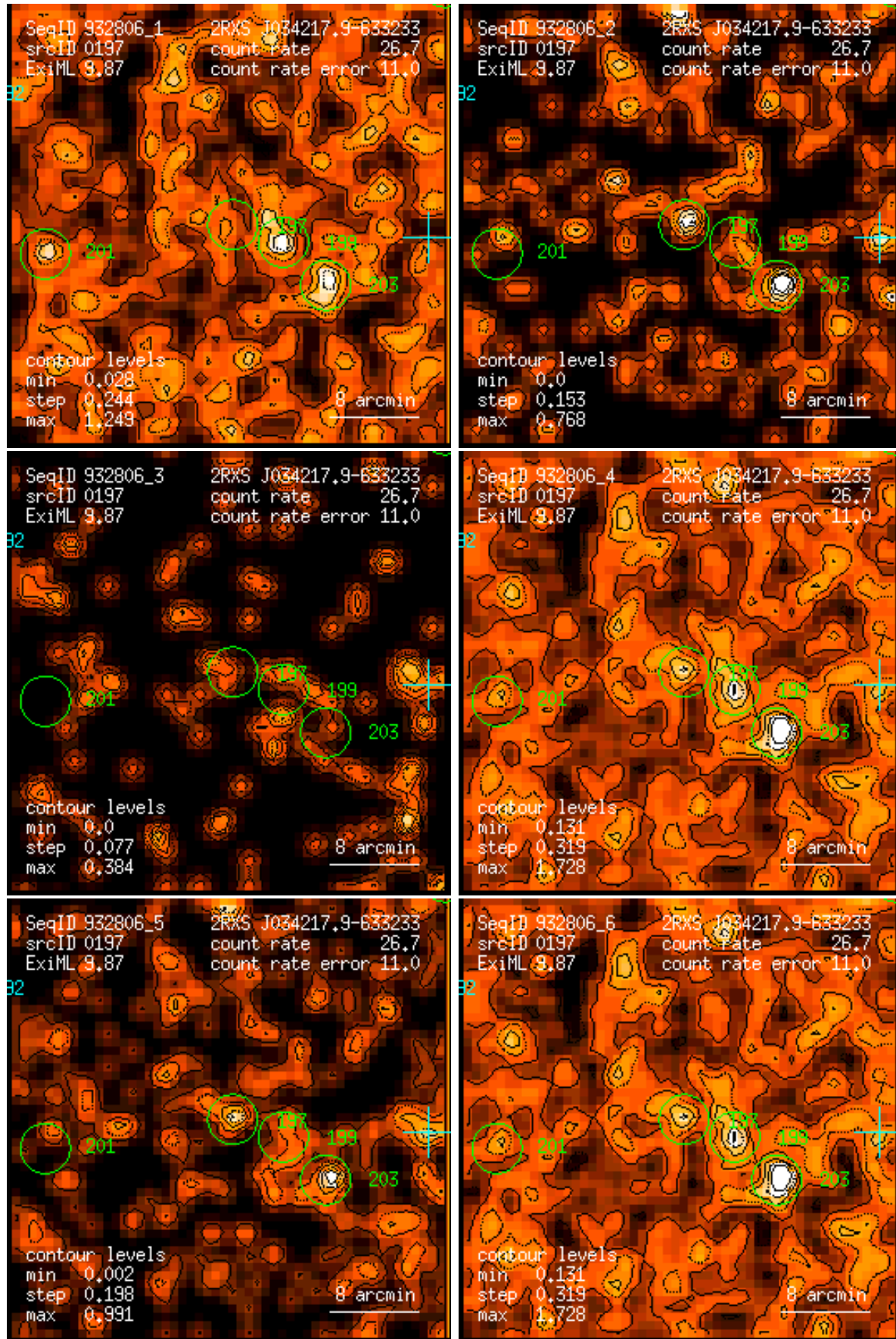
Figure 197: RASS 932806: detection 0197: band rate images, Gaussian filter: (1) PSPC channels 11 – 41, (2) 52 – 90, (3) 91 – 201, (4) 11 – 235, (5) 52 – 201, (6) 11 – 201. Broad band rates in counts/ks. Band rate contour levels in counts/ks/arcmin 2 .
