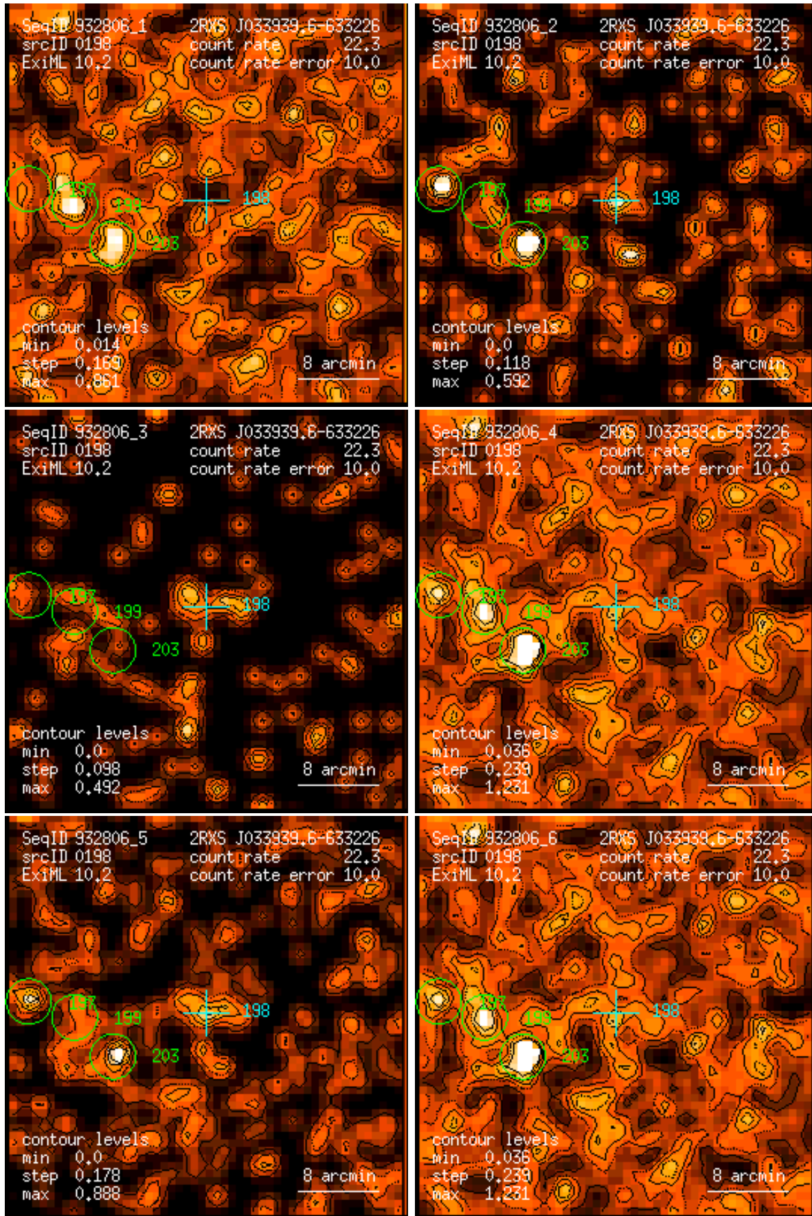
Figure 198: RASS 932806: detection 0198: band rate images, Gaussian filter: (1) PSPC channels 11 – 41, (2) 52 – 90, (3) 91 – 201, (4) 11 – 235, (5) 52 – 201, (6) 11 – 201. Broad band rates in counts/ks. Band rate contour levels in counts/ks/arcmin 2 .
