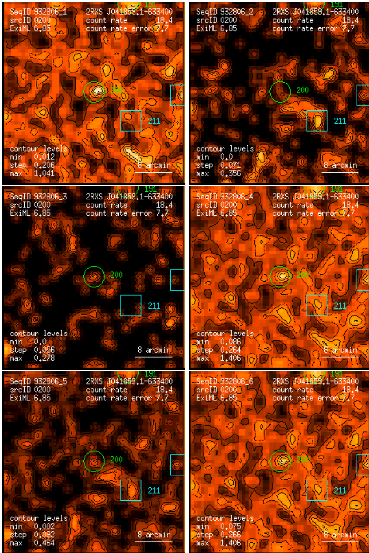
Figure 200: RASS 932806: detection 0200: band rate images, Gaussian filter: (1) PSPC channels 11 – 41, (2) 52 – 90, (3) 91 – 201, (4) 11 – 235, (5) 52 – 201, (6) 11 – 201. Broad band rates in counts/ks. Band rate contour levels in counts/ks/arcmin 2 .
