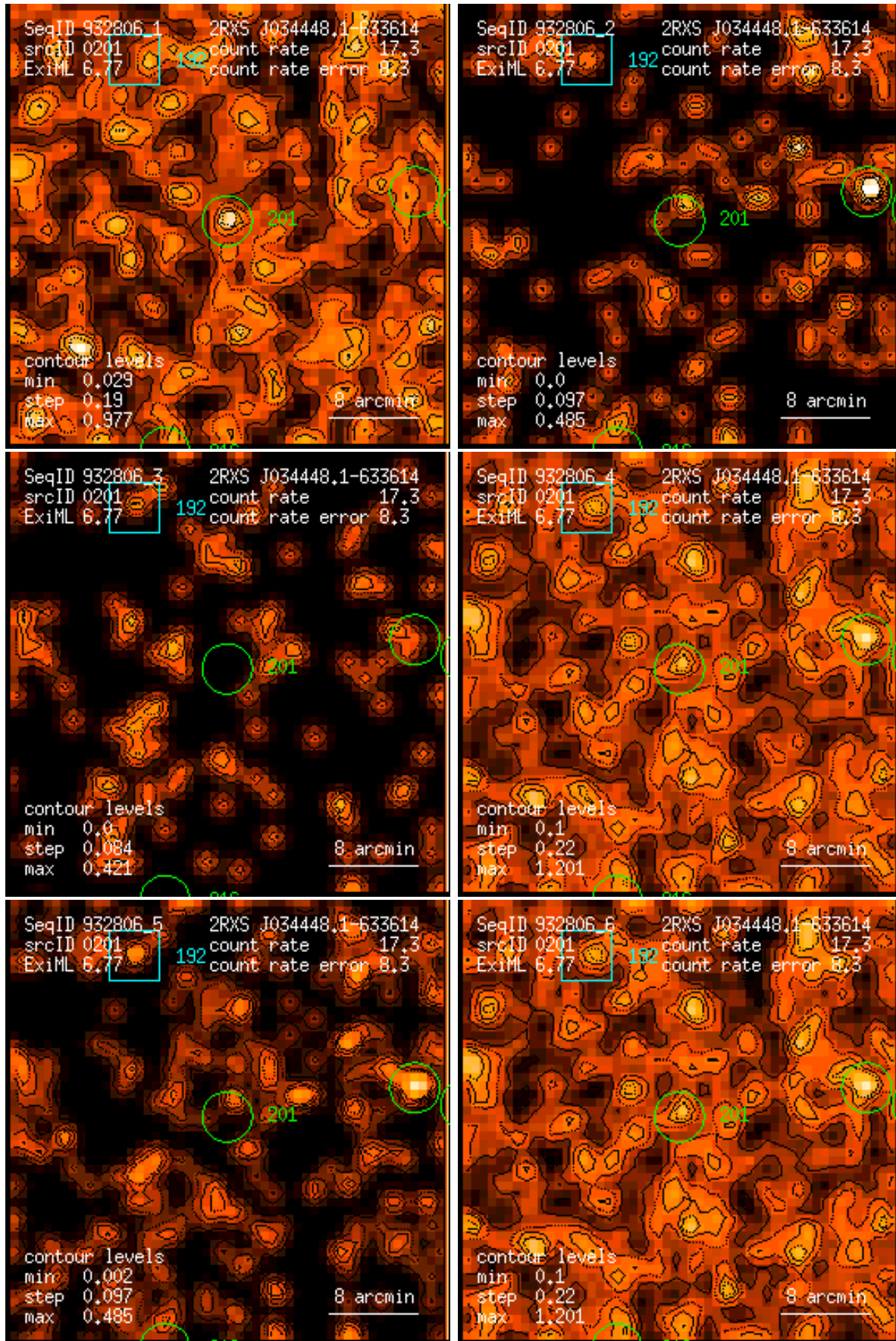
Figure 201: RASS 932806: detection 0201: band rate images, Gaussian filter: (1) PSPC channels 11 – 41, (2) 52 – 90, (3) 91 – 201, (4) 11 – 235, (5) 52 – 201, (6) 11 – 201. Broad band rates in counts/ks. Band rate contour levels in counts/ks/arcmin 2 .
