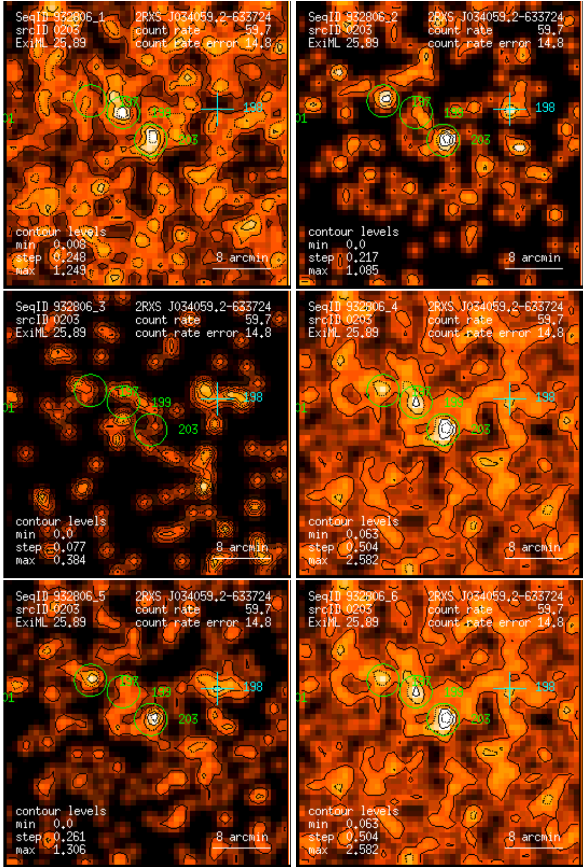
Figure 203: RASS 932806: detection 0203: band rate images, Gaussian filter: (1) PSPC channels 11 – 41, (2) 52 – 90, (3) 91 – 201, (4) 11 – 235, (5) 52 – 201, (6) 11 – 201. Broad band rates in counts/ks. Band rate contour levels in counts/ks/arcmin 2 .
