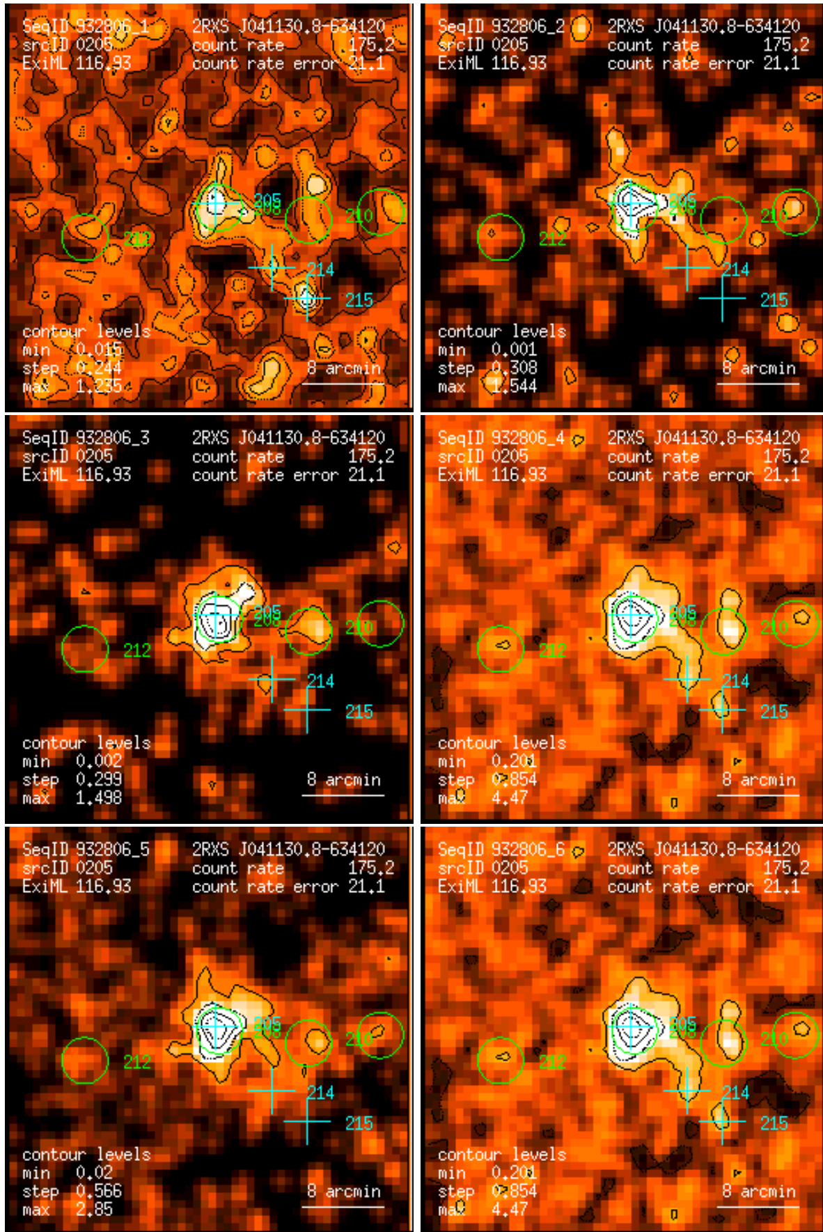
Figure 205: RASS 932806: detection 0205: band rate images, Gaussian filter: (1) PSPC channels 11 – 41, (2) 52 – 90, (3) 91 – 201, (4) 11 – 235, (5) 52 – 201, (6) 11 – 201. Broad band rates in counts/ks. Band rate contour levels in counts/ks/arcmin 2 .
