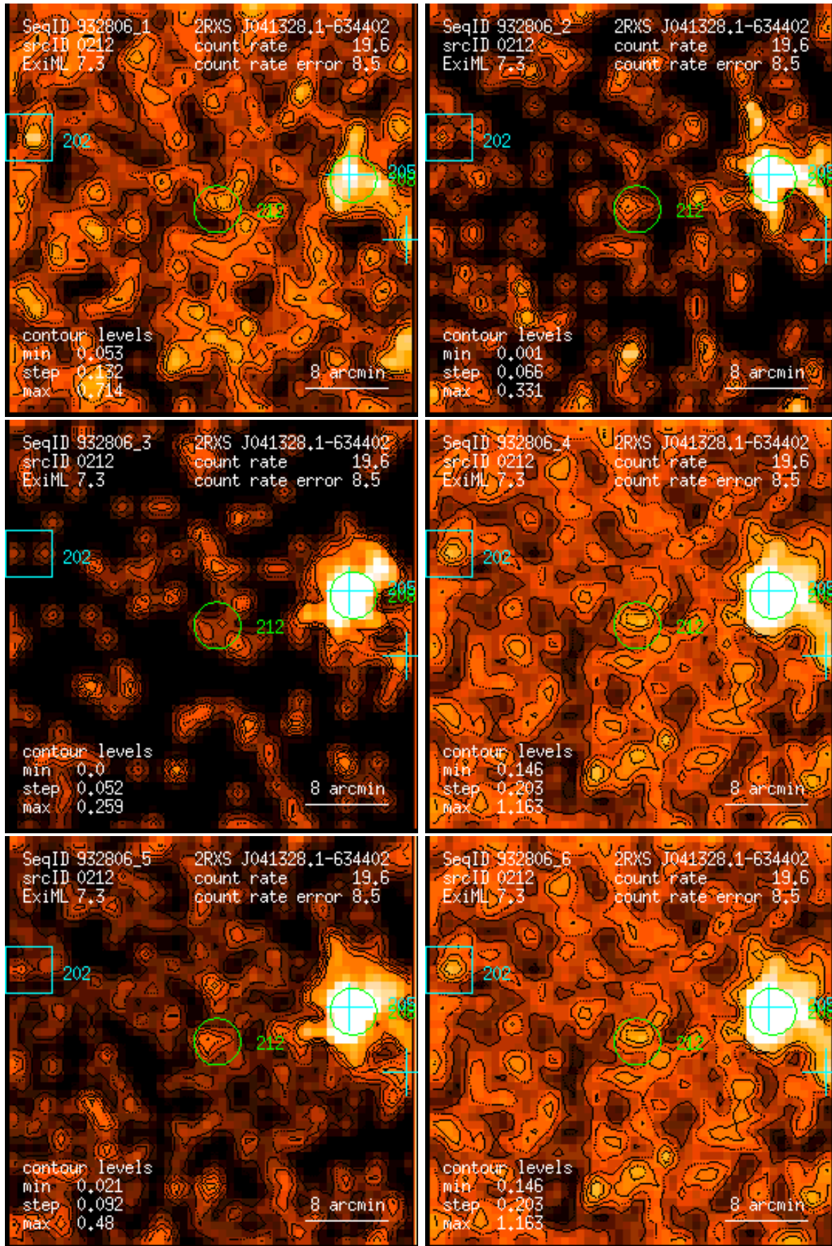
Figure 212: RASS 932806: detection 0212: band rate images, Gaussian filter: (1) PSPC channels 11 – 41, (2) 52 – 90, (3) 91 – 201, (4) 11 – 235, (5) 52 – 201, (6) 11 – 201. Broad band rates in counts/ks. Band rate contour levels in counts/ks/arcmin 2 .
