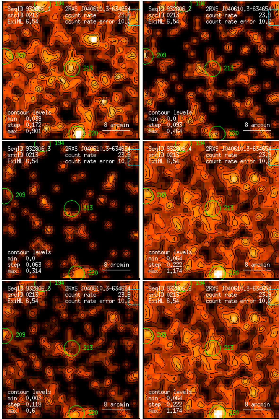
Figure 213: RASS 932806: detection 0213: band rate images, Gaussian filter: (1) PSPC channels 11 – 41, (2) 52 – 90, (3) 91 – 201, (4) 11 – 235, (5) 52 – 201, (6) 11 – 201. Broad band rates in counts/ks. Band rate contour levels in counts/ks/arcmin 2 .
