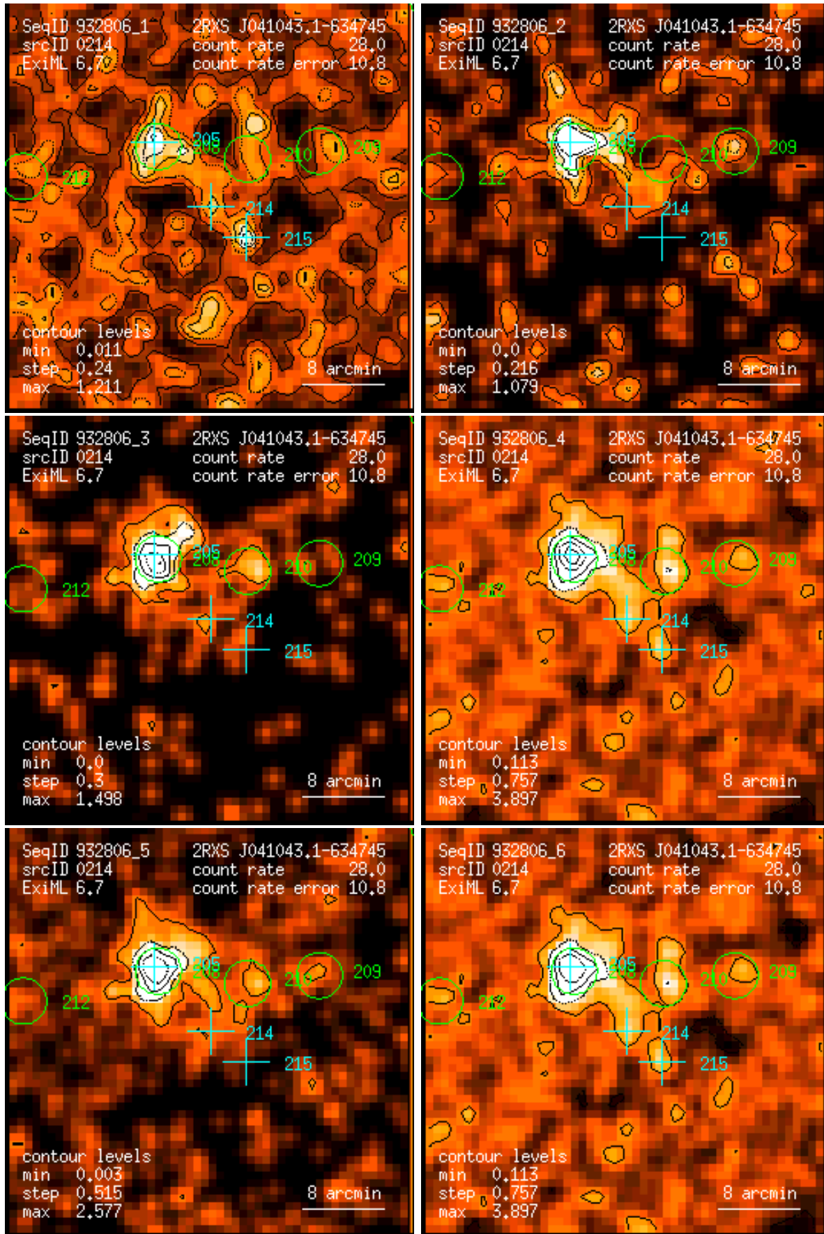
Figure 214: RASS 932806: detection 0214: band rate images, Gaussian filter: (1) PSPC channels 11 – 41, (2) 52 – 90, (3) 91 – 201, (4) 11 – 235, (5) 52 – 201, (6) 11 – 201. Broad band rates in counts/ks. Band rate contour levels in counts/ks/arcmin 2 .
