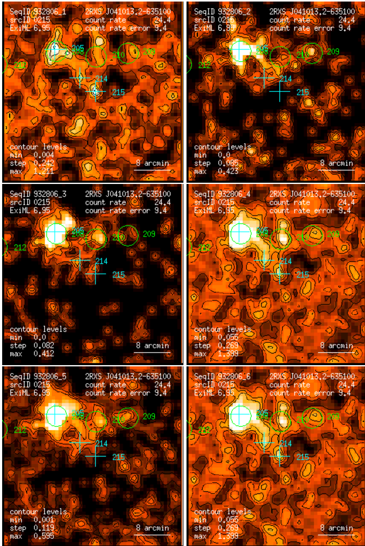
Figure 215: RASS 932806: detection 0215: band rate images, Gaussian filter: (1) PSPC channels 11 – 41, (2) 52 – 90, (3) 91 – 201, (4) 11 – 235, (5) 52 – 201, (6) 11 – 201. Broad band rates in counts/ks. Band rate contour levels in counts/ks/arcmin 2 .
