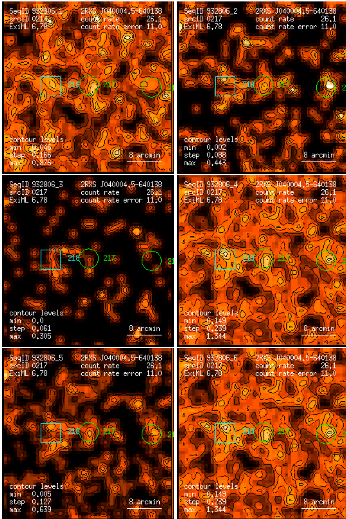
Figure 217: RASS 932806: detection 0217: band rate images, Gaussian filter: (1) PSPC channels 11 – 41, (2) 52 – 90, (3) 91 – 201, (4) 11 – 235, (5) 52 – 201, (6) 11 – 201. Broad band rates in counts/ks. Band rate contour levels in counts/ks/arcmin 2 .
