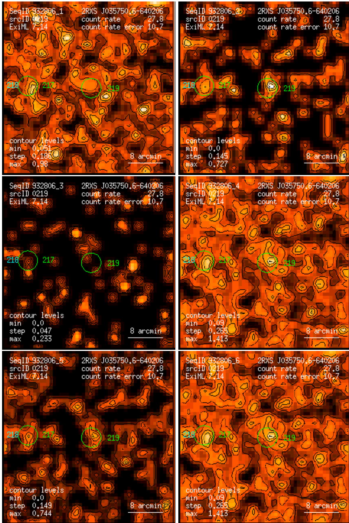
Figure 219: RASS 932806: detection 0219: band rate images, Gaussian filter: (1) PSPC channels 11 – 41, (2) 52 – 90, (3) 91 – 201, (4) 11 – 235, (5) 52 – 201, (6) 11 – 201. Broad band rates in counts/ks. Band rate contour levels in counts/ks/arcmin 2 .
