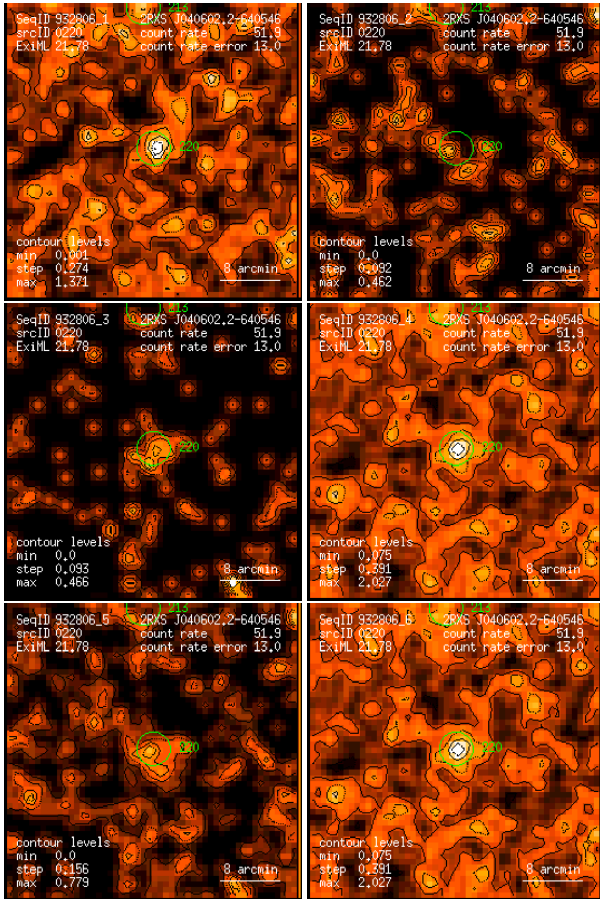
Figure 220: RASS 932806: detection 0220: band rate images, Gaussian filter: (1) PSPC channels 11 – 41, (2) 52 – 90, (3) 91 – 201, (4) 11 – 235, (5) 52 – 201, (6) 11 – 201. Broad band rates in counts/ks. Band rate contour levels in counts/ks/arcmin 2 .
