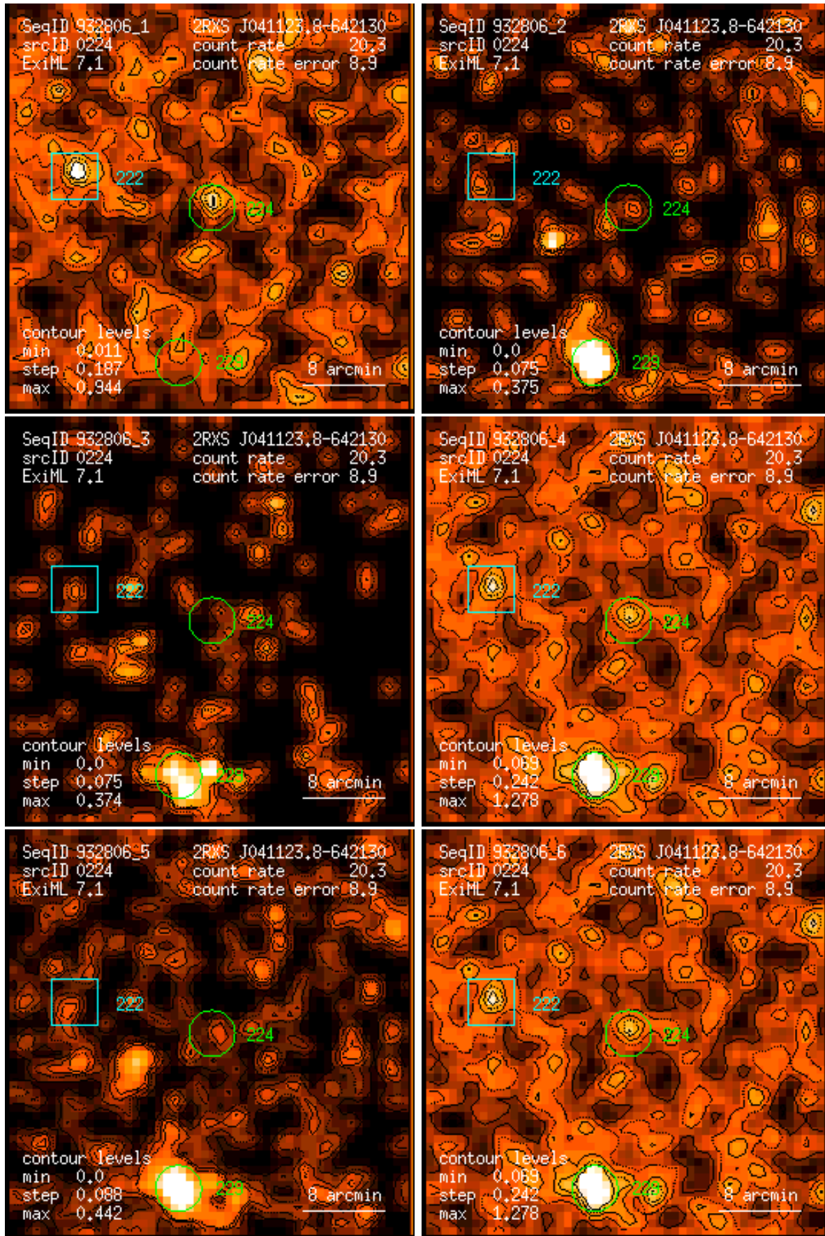
Figure 224: RASS 932806: detection 0224: band rate images, Gaussian filter: (1) PSPC channels 11 – 41, (2) 52 – 90, (3) 91 – 201, (4) 11 – 235, (5) 52 – 201, (6) 11 – 201. Broad band rates in counts/ks. Band rate contour levels in counts/ks/arcmin 2 .
