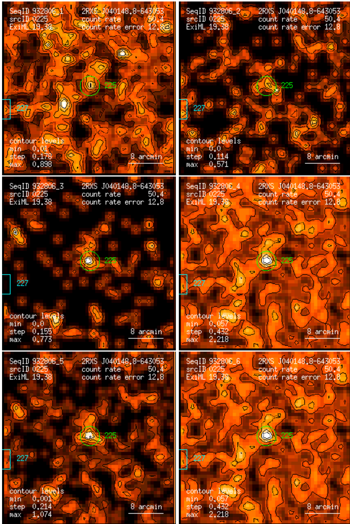
Figure 225: RASS 932806: detection 0225: band rate images, Gaussian filter: (1) PSPC channels 11 – 41, (2) 52 – 90, (3) 91 – 201, (4) 11 – 235, (5) 52 – 201, (6) 11 – 201. Broad band rates in counts/ks. Band rate contour levels in counts/ks/arcmin 2 .
