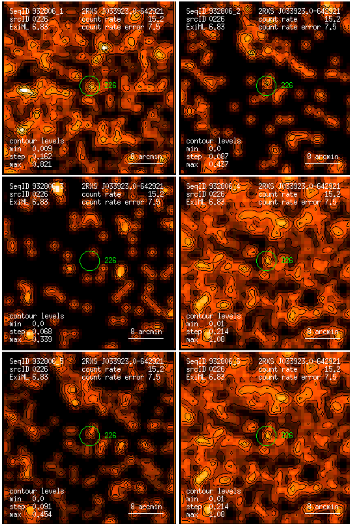
Figure 226: RASS 932806: detection 0226: band rate images, Gaussian filter: (1) PSPC channels 11 – 41, (2) 52 – 90, (3) 91 – 201, (4) 11 – 235, (5) 52 – 201, (6) 11 – 201. Broad band rates in counts/ks. Band rate contour levels in counts/ks/arcmin 2 .
