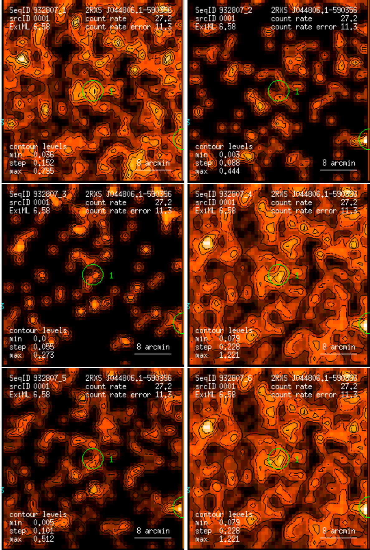
Figure 1: RASS 932807: detection 0001: band rate images, Gaussian filter: (1) PSPC channels 11 – 41, (2) 52 – 90, (3) 91 – 201, (4) 11 – 235, (5) 52 – 201, (6) 11 – 201. Broad band rates in counts/ks. Band rate contour levels in counts/ks/arcmin 2 .
