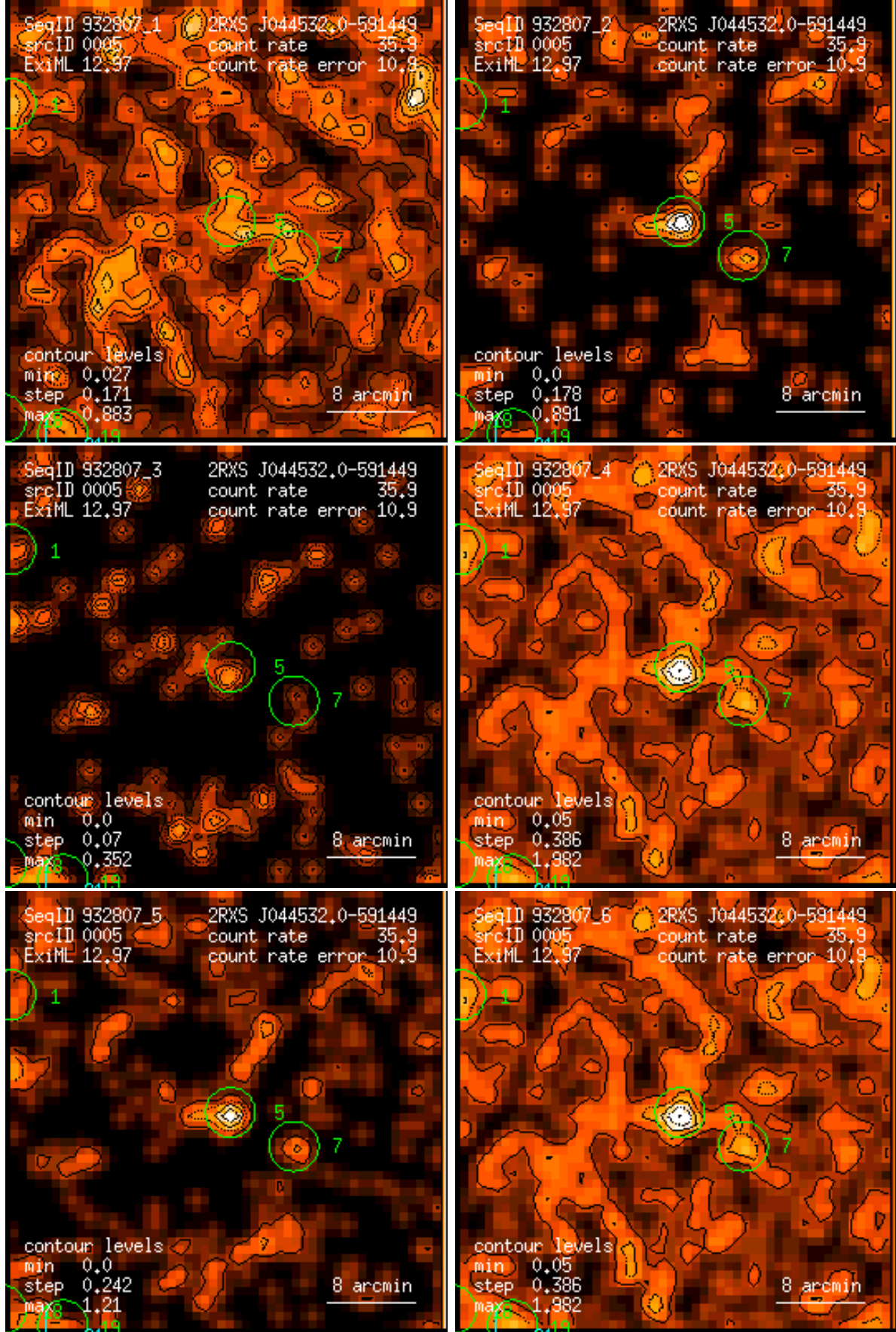
Figure 5: RASS 932807: detection 0005: band rate images, Gaussian filter: (1) PSPC channels 11 – 41, (2) 52 – 90, (3) 91 – 201, (4) 11 – 235, (5) 52 – 201, (6) 11 – 201. Broad band rates in counts/ks. Band rate contour levels in counts/ks/arcmin 2 .
