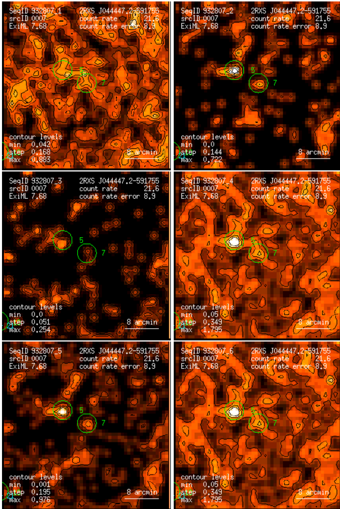
Figure 7: RASS 932807: detection 0007: band rate images, Gaussian filter: (1) PSPC channels 11 – 41, (2) 52 – 90, (3) 91 – 201, (4) 11 – 235, (5) 52 – 201, (6) 11 – 201. Broad band rates in counts/ks. Band rate contour levels in counts/ks/arcmin 2 .
