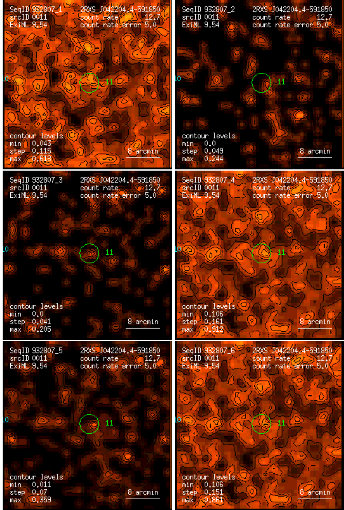
Figure 11: RASS 932807: detection 0011: band rate images, Gaussian filter: (1) PSPC channels 11 – 41, (2) 52 – 90, (3) 91 – 201, (4) 11 – 235, (5) 52 – 201, (6) 11 – 201. Broad band rates in counts/ks. Band rate contour levels in counts/ks/arcmin 2 .
