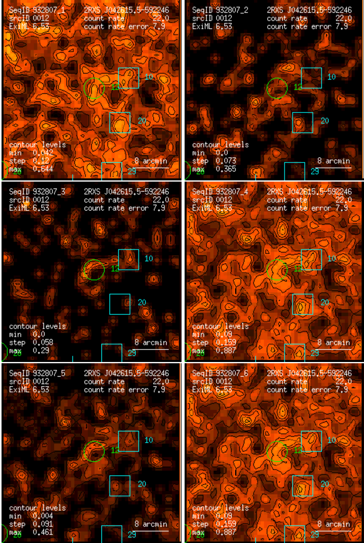
Figure 12: RASS 932807: detection 0012: band rate images, Gaussian filter: (1) PSPC channels 11 – 41, (2) 52 – 90, (3) 91 – 201, (4) 11 – 235, (5) 52 – 201, (6) 11 – 201. Broad band rates in counts/ks. Band rate contour levels in counts/ks/arcmin 2 .
