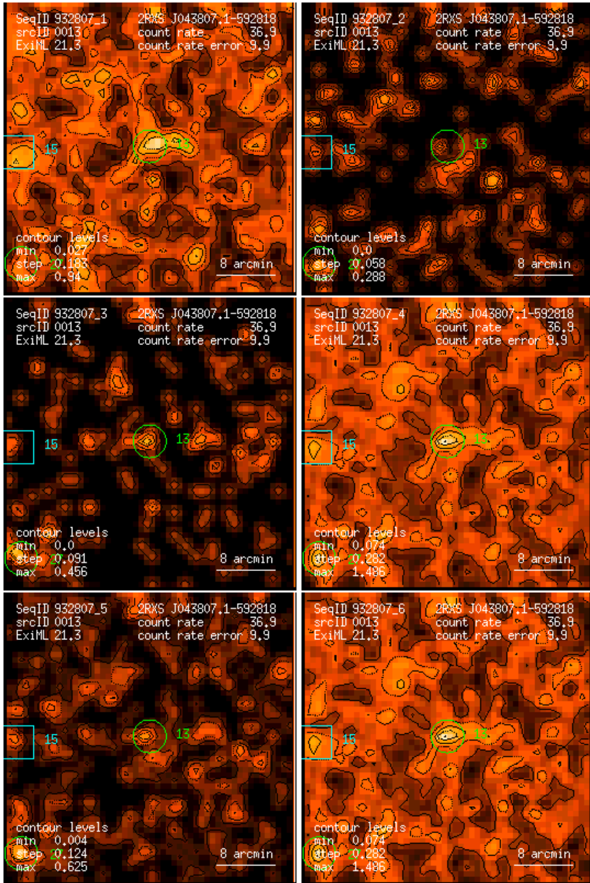
Figure 13: RASS 932807: detection 0013: band rate images, Gaussian filter: (1) PSPC channels 11 – 41, (2) 52 – 90, (3) 91 – 201, (4) 11 – 235, (5) 52 – 201, (6) 11 – 201. Broad band rates in counts/ks. Band rate contour levels in counts/ks/arcmin 2 .
