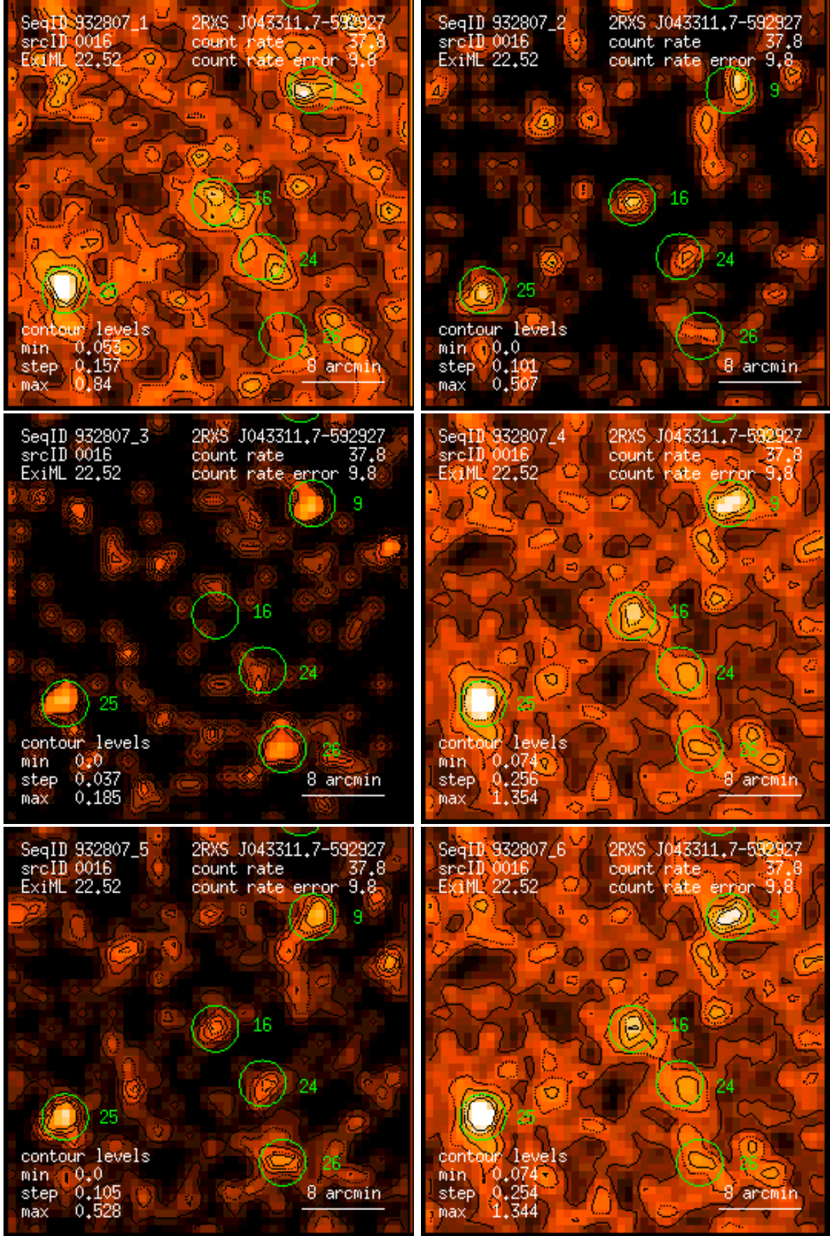
Figure 16: RASS 932807: detection 0016: band rate images, Gaussian filter: (1) PSPC channels 11 – 41, (2) 52 – 90, (3) 91 – 201, (4) 11 – 235, (5) 52 – 201, (6) 11 – 201. Broad band rates in counts/ks. Band rate contour levels in counts/ks/arcmin 2 .
