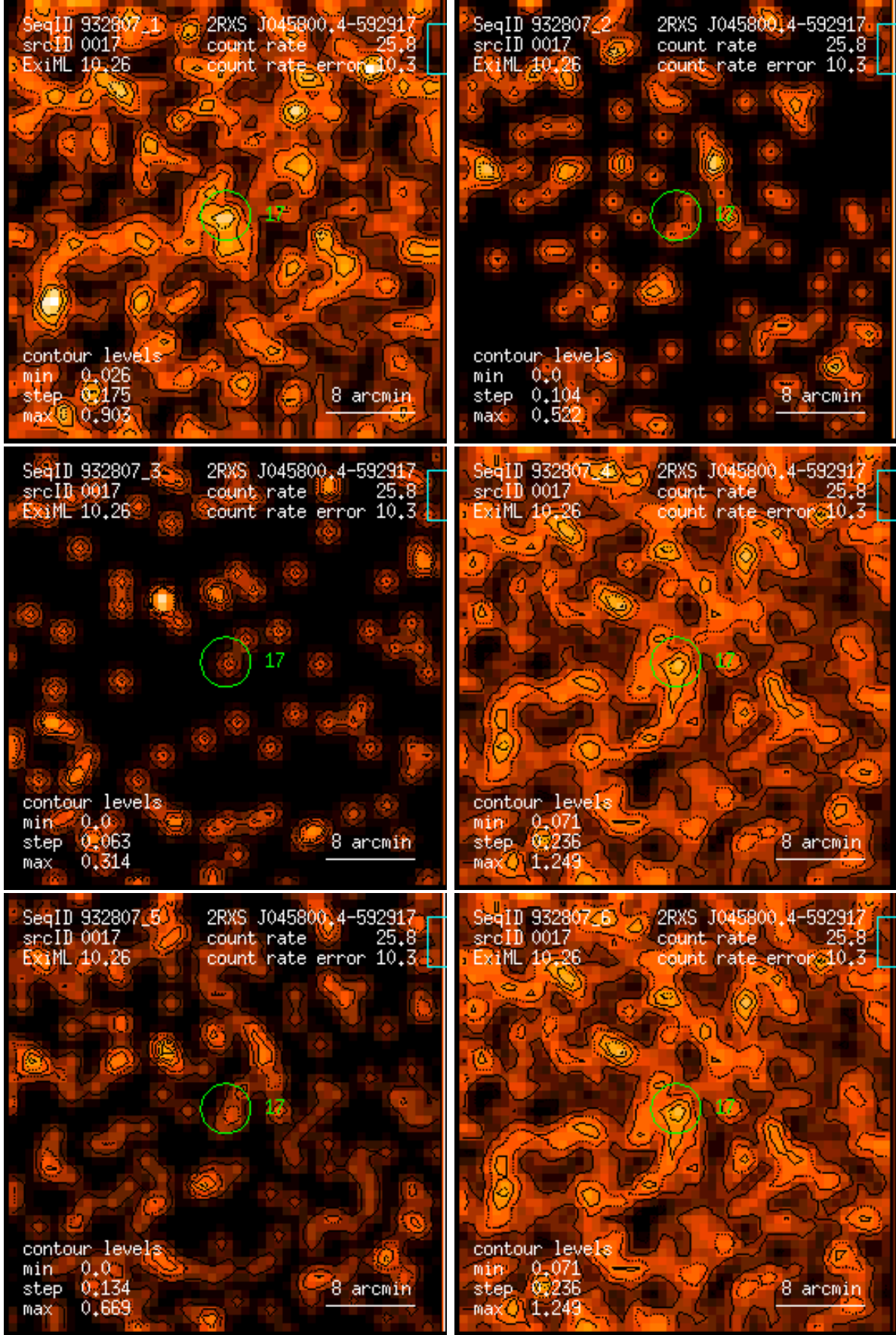
Figure 17: RASS 932807: detection 0017: band rate images, Gaussian filter: (1) PSPC channels 11 – 41, (2) 52 – 90, (3) 91 – 201, (4) 11 – 235, (5) 52 – 201, (6) 11 – 201. Broad band rates in counts/ks. Band rate contour levels in counts/ks/arcmin 2 .
