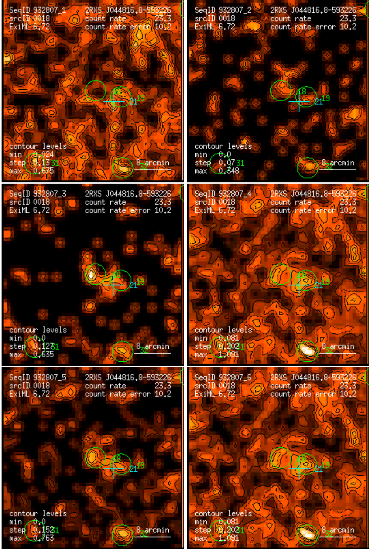
Figure 18: RASS 932807: detection 0018: band rate images, Gaussian filter: (1) PSPC channels 11 – 41, (2) 52 – 90, (3) 91 – 201, (4) 11 – 235, (5) 52 – 201, (6) 11 – 201. Broad band rates in counts/ks. Band rate contour levels in counts/ks/arcmin 2 .
