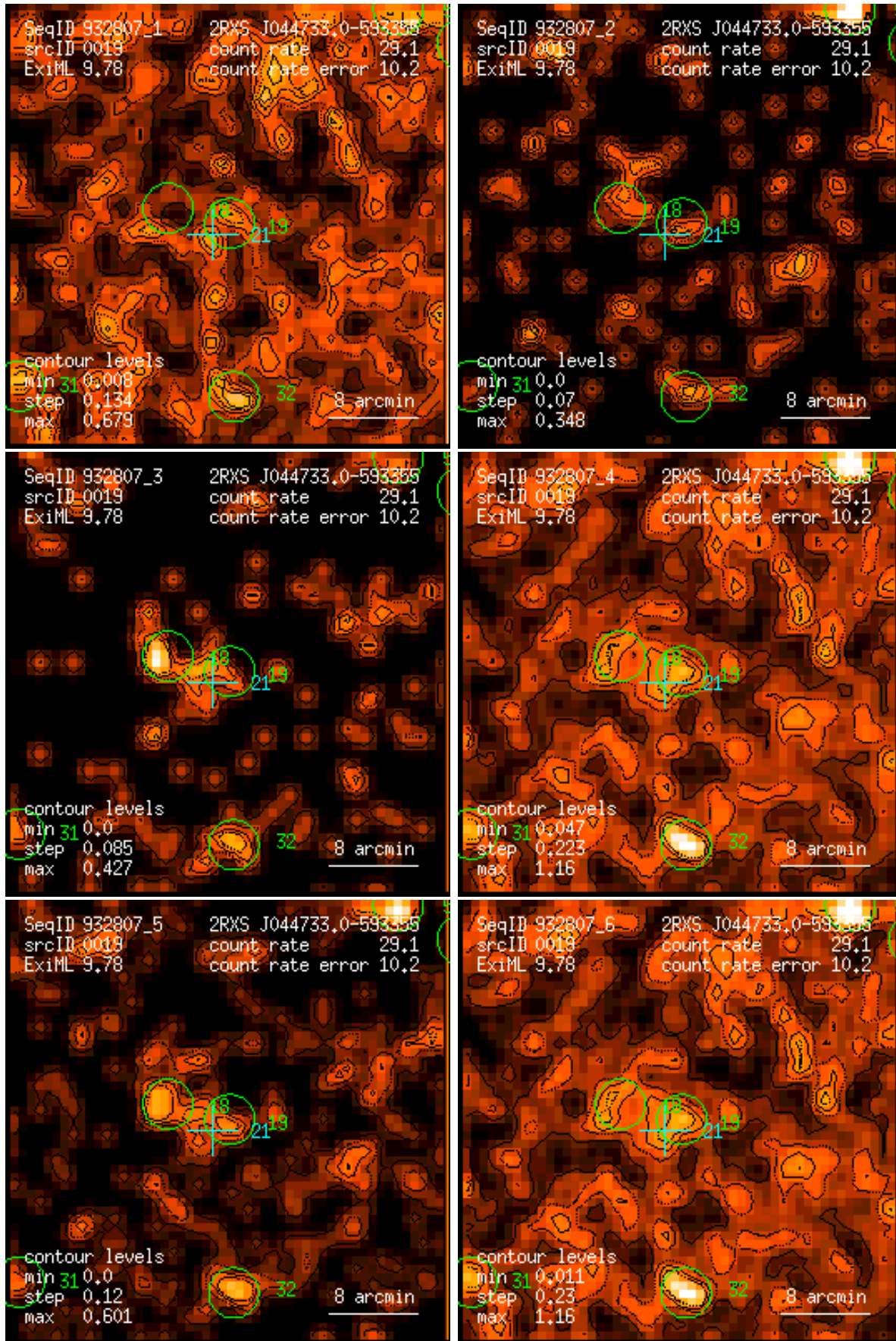
Figure 19: RASS 932807: detection 0019: band rate images, Gaussian filter: (1) PSPC channels 11 – 41, (2) 52 – 90, (3) 91 – 201, (4) 11 – 235, (5) 52 – 201, (6) 11 – 201. Broad band rates in counts/ks. Band rate contour levels in counts/ks/arcmin 2 .
