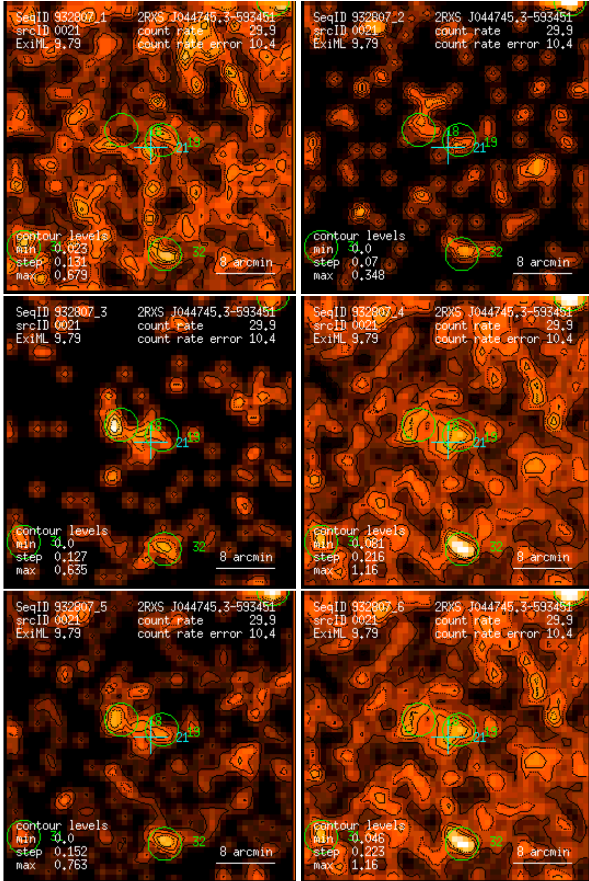
Figure 21: RASS 932807: detection 0021: band rate images, Gaussian filter: (1) PSPC channels 11 – 41, (2) 52 – 90, (3) 91 – 201, (4) 11 – 235, (5) 52 – 201, (6) 11 – 201. Broad band rates in counts/ks. Band rate contour levels in counts/ks/arcmin 2 .
