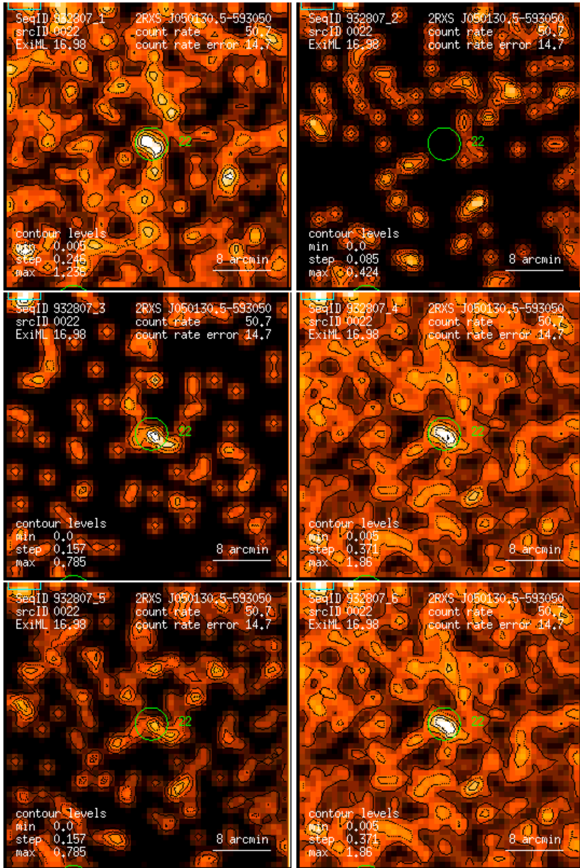
Figure 22: RASS 932807: detection 0022: band rate images, Gaussian filter: (1) PSPC channels 11 – 41, (2) 52 – 90, (3) 91 – 201, (4) 11 – 235, (5) 52 – 201, (6) 11 – 201. Broad band rates in counts/ks. Band rate contour levels in counts/ks/arcmin 2 .
